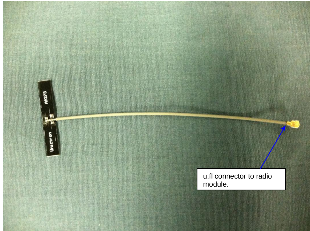
Figure 4 - Dipole Antenna
