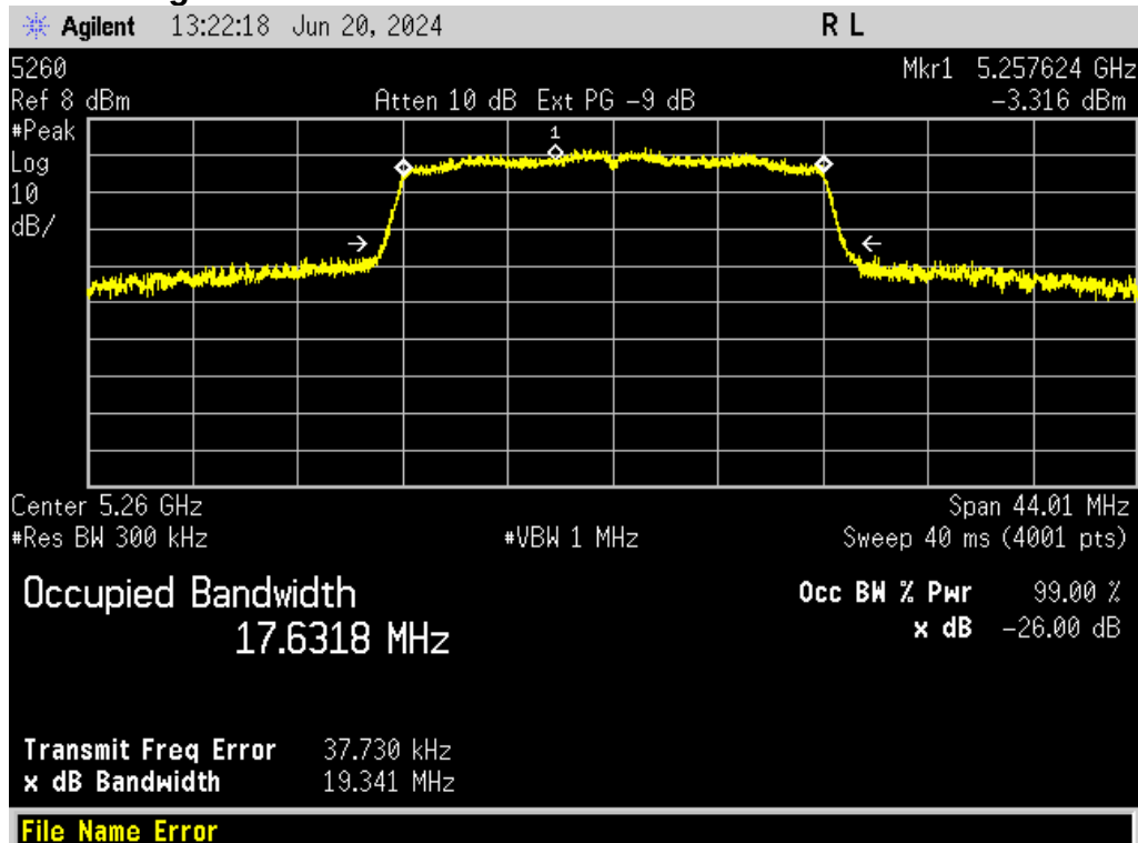
Figure 18. 26 dB BW and OBW -802.11n- Channel 52
