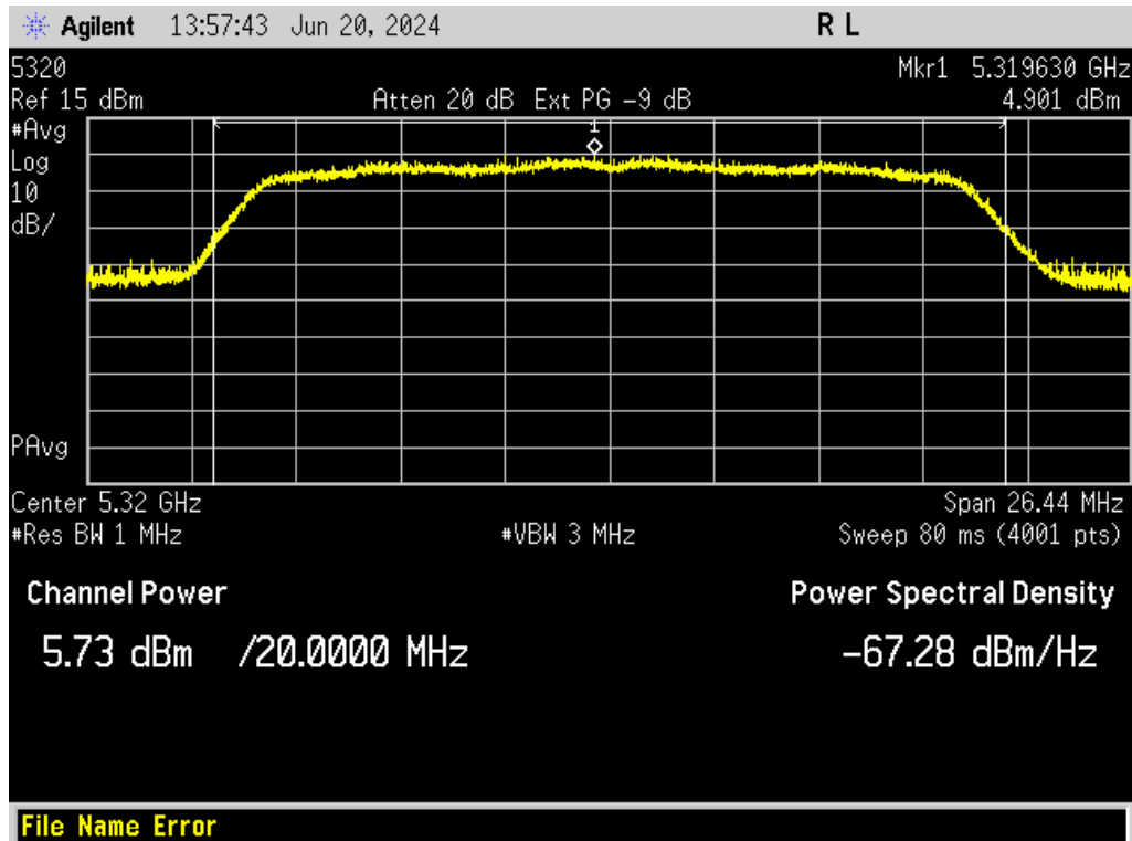
Figure 31. Antenna Conducted Output Power, 802.11a Channel 64
