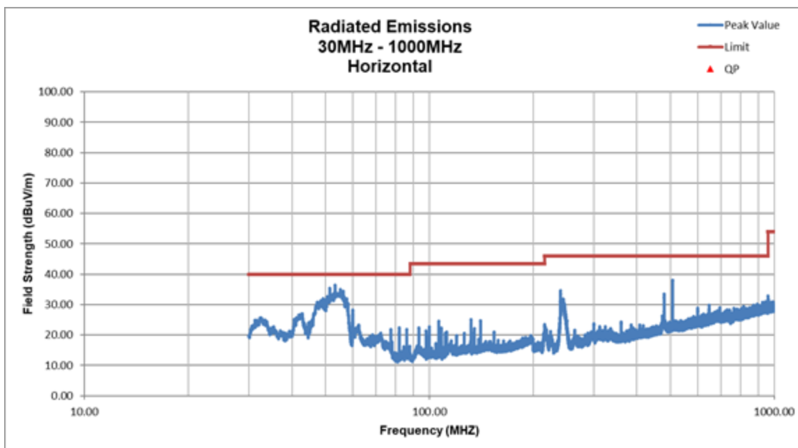
Figure 41. Radiated Emissions, Horizontal 30 – 1000 MHz
