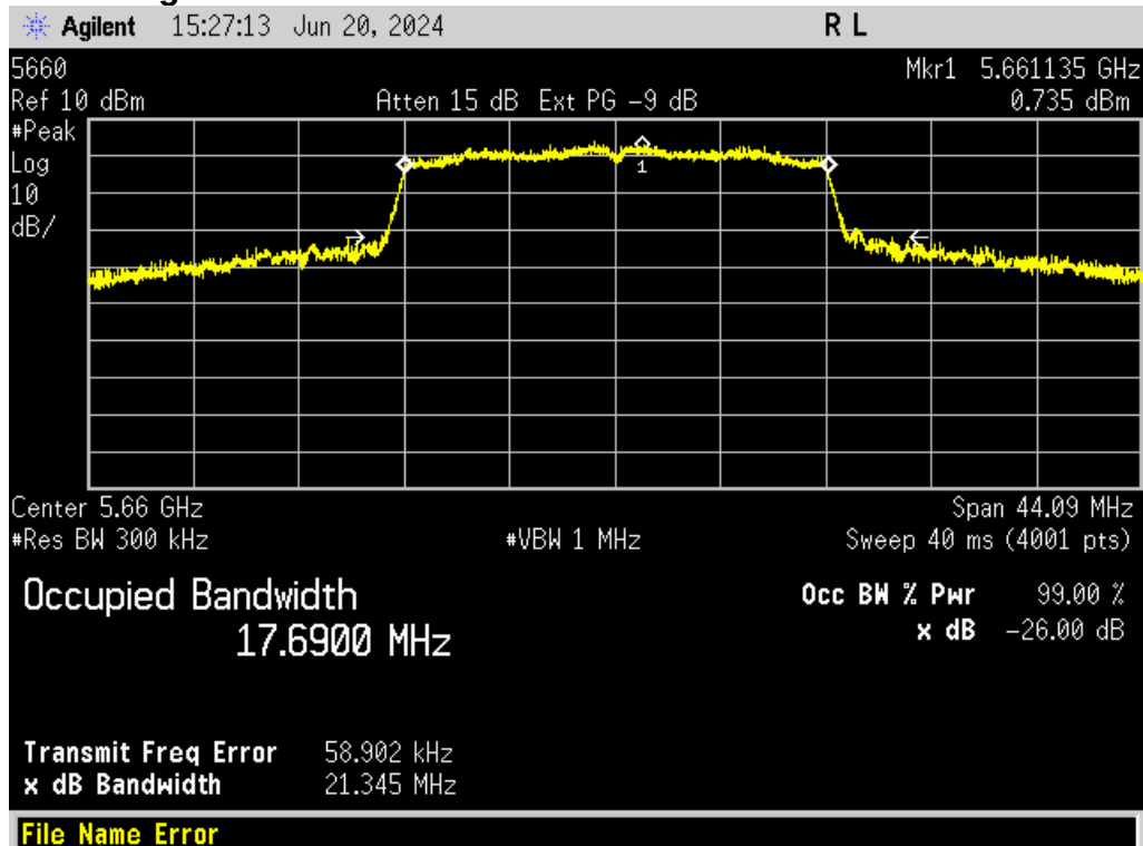
Figure 26. 26 dB BW and OBW -802.11n- Channel 132
