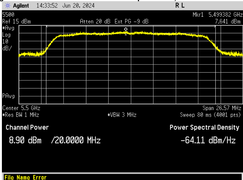
Figure 34. Peak Antenna Conducted Output Power, 802.11n Channel 100
