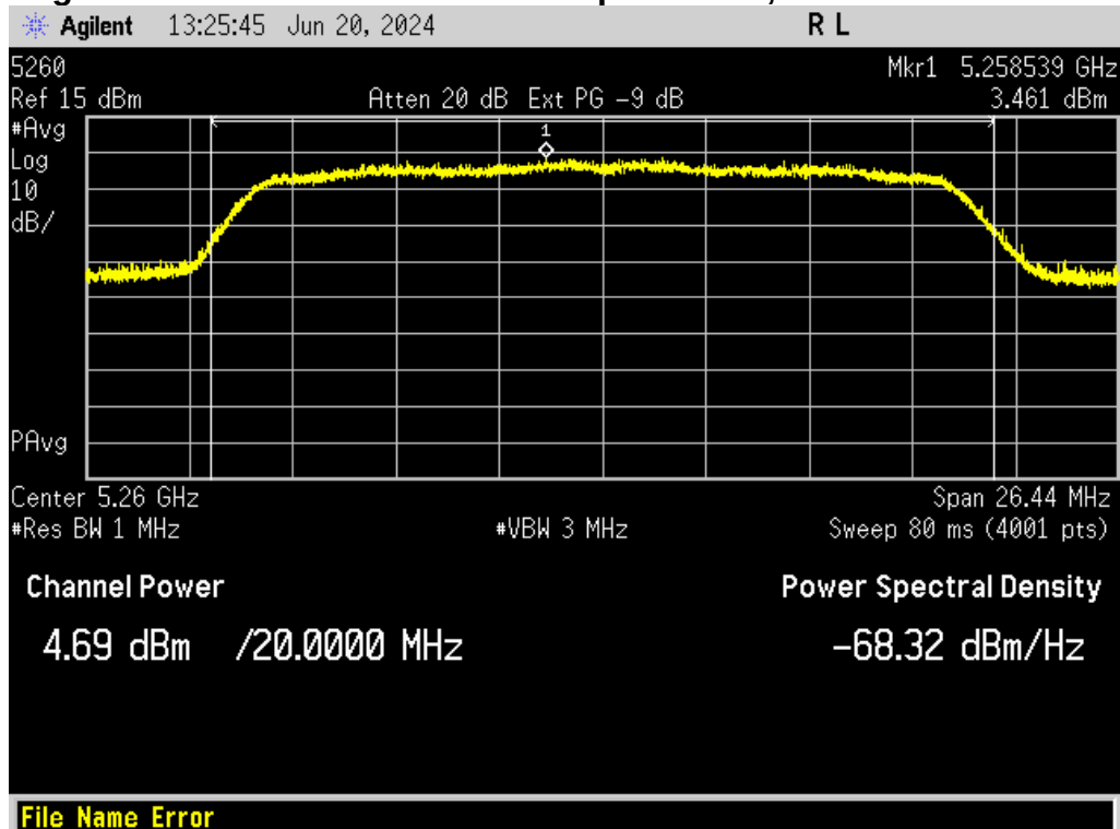
Figure 30. Antenna Conducted Output Power, 802.11n Channel 52
