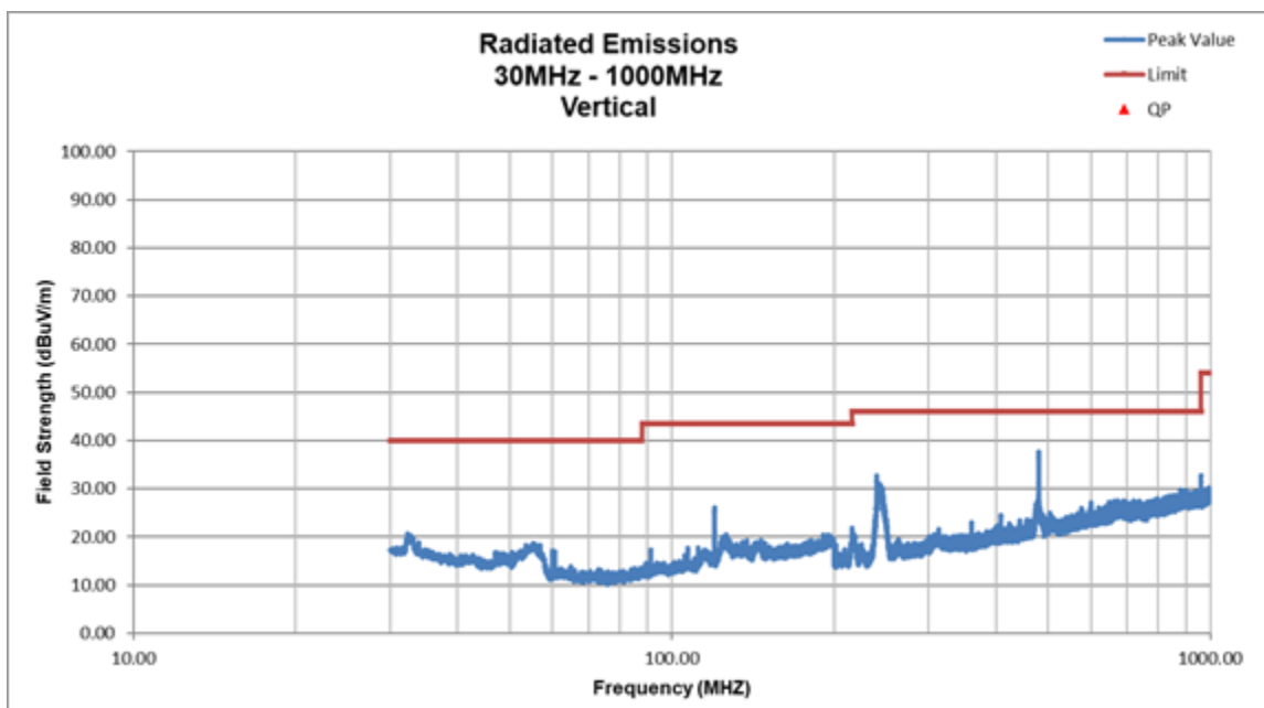
Figure 42. Radiated Emissions, Vertical 30 – 1000 MHz
