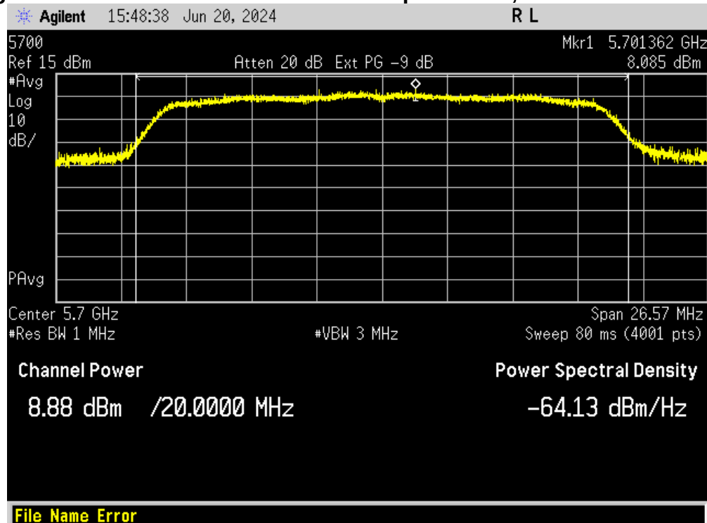
Figure 40. Peak Antenna Conducted Output Power, 802.11n Channel 140
