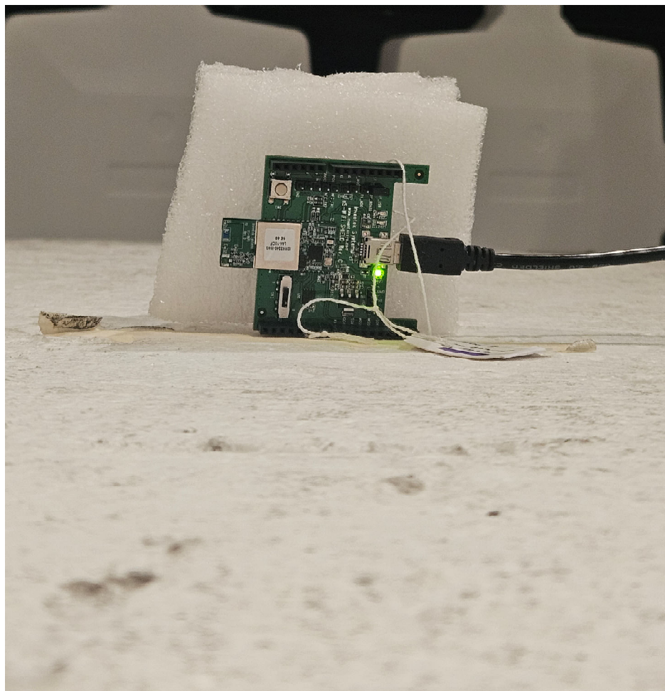
Figure 1. Radiated Emissions Test Setup, Front
