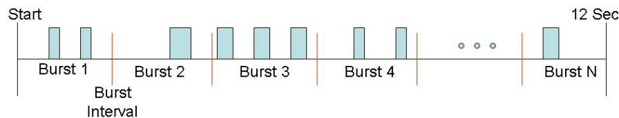
Figure 15. Long Pulse Radar Test Signal Waveform
