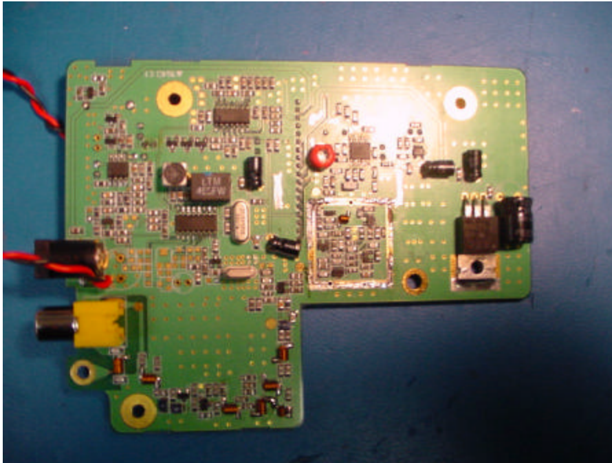
RF PCB bottom with shield removed
