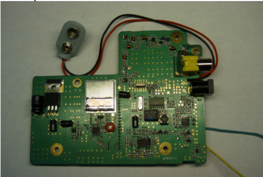
RF PCB bottom With Shield
