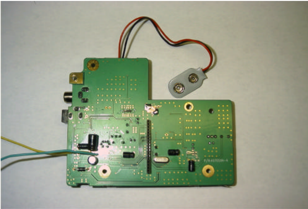
RF PCB top
