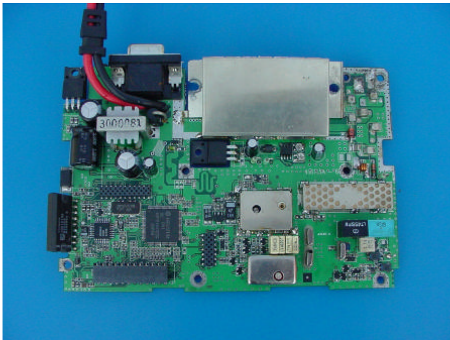
19.1.5 MAIN PCB TOP
