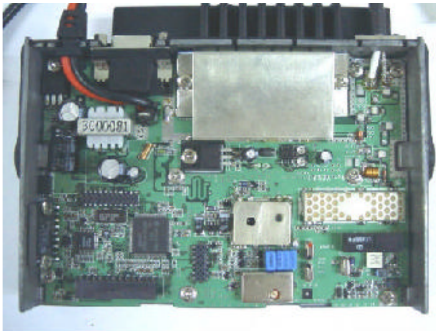
19.1.6 TOP PCB INSIDE CASE
