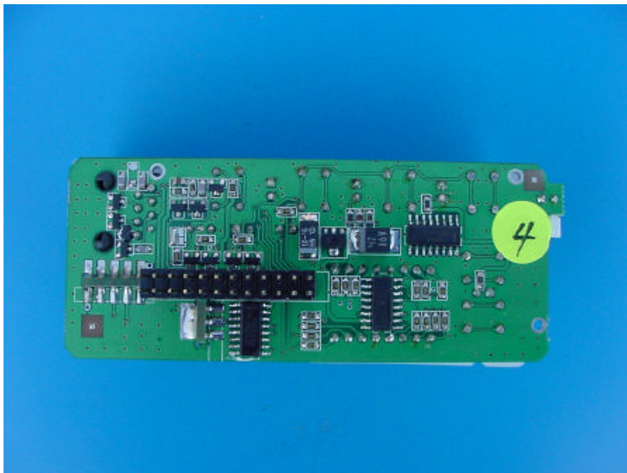
19.1.1 BACK OF FRONT PCB
