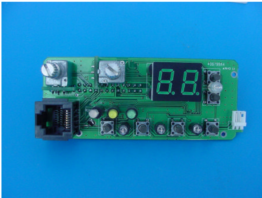
19.1.3 FRONT OF FRONT PCB
