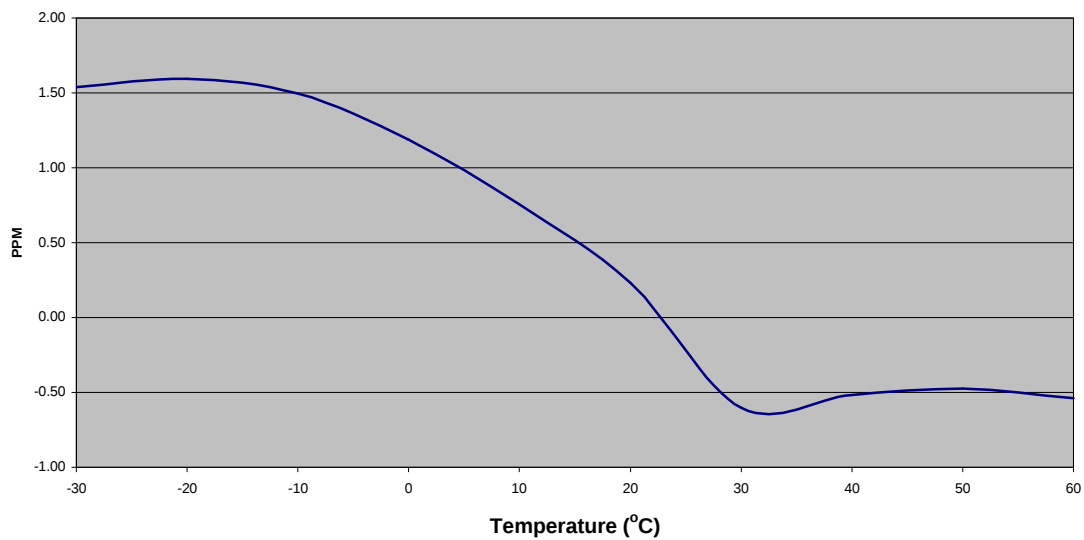
Frequency Stability (Channel 8; 25 kHz Channel Spacing; 10 W)
