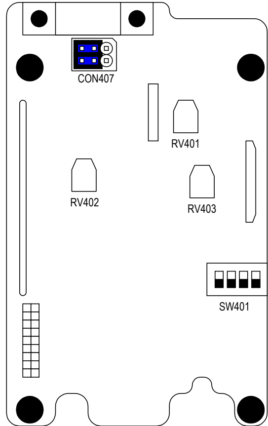
DIGITAL BOARD ALIGNMENT POINTS
