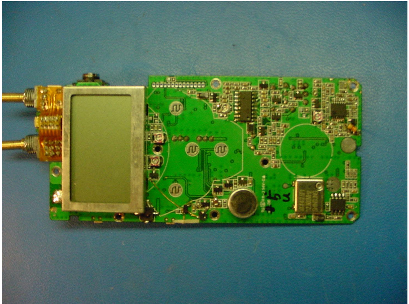
PHOTOGRAPH 11: FRONT VIEW OF PCB BOARD
