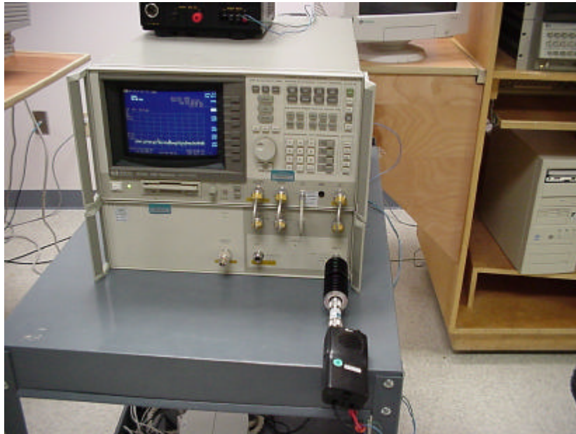
Antenna Conducted Emissions/Mask test setup
