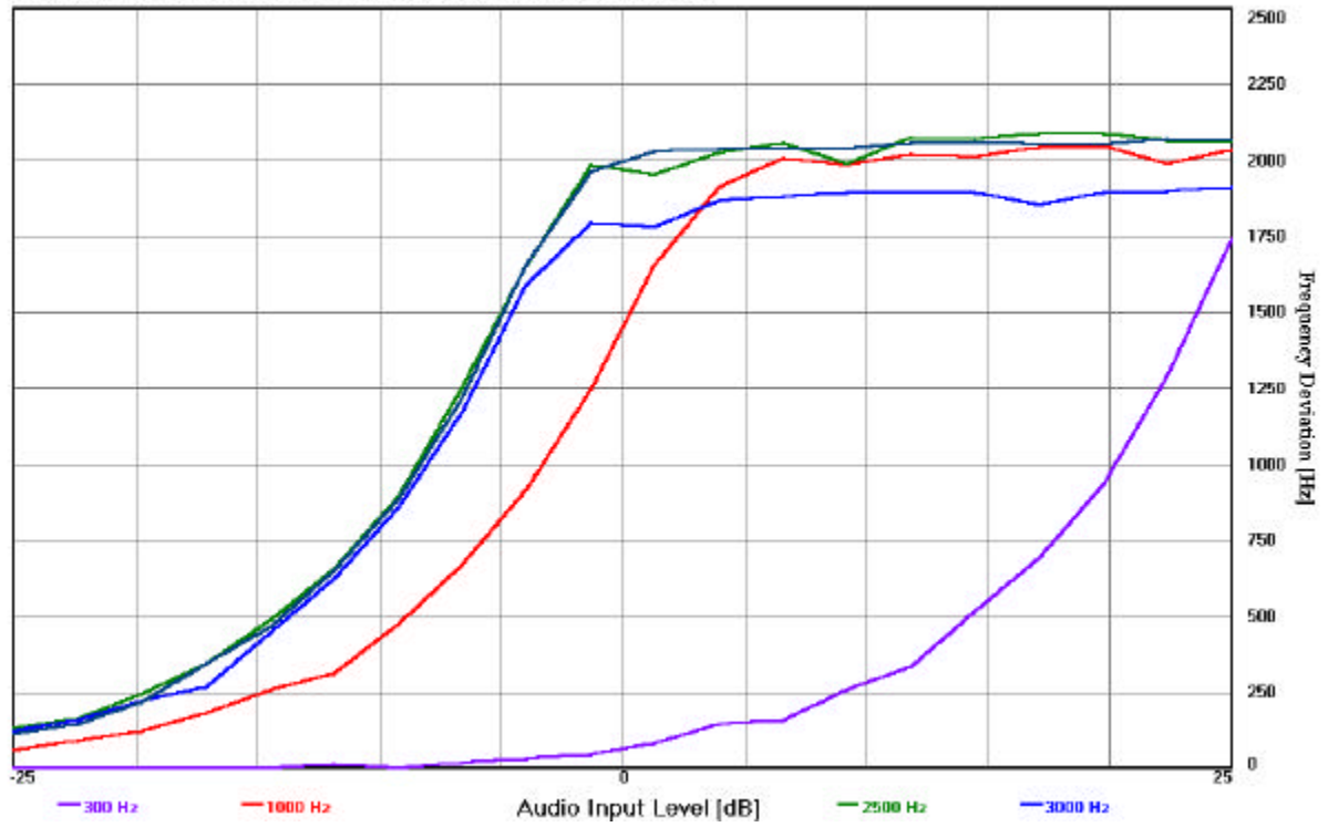
RTL Modulation Limiting Response (151.82 MHz : 11.25 kHz Channel Spacing) Negative Peak
