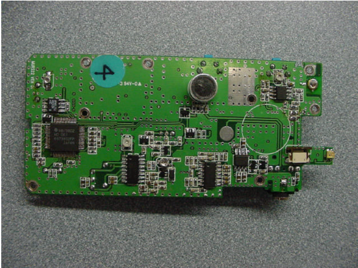
Back of PCB
