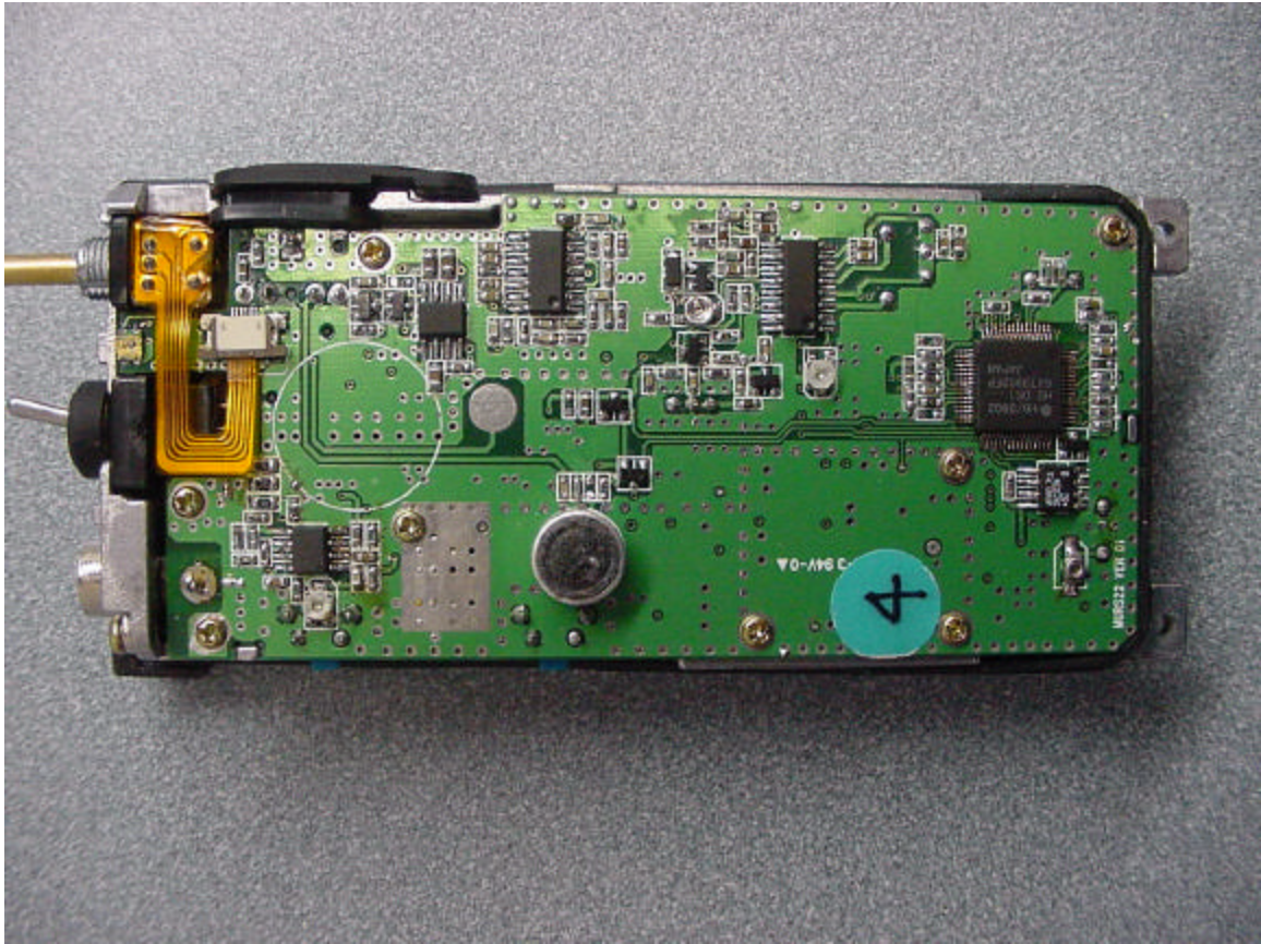
Front of PCB in Chassis
