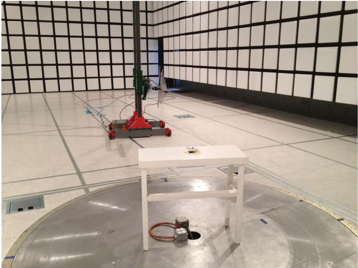
Radiated Field Strength Spurious Emission Test Setup
