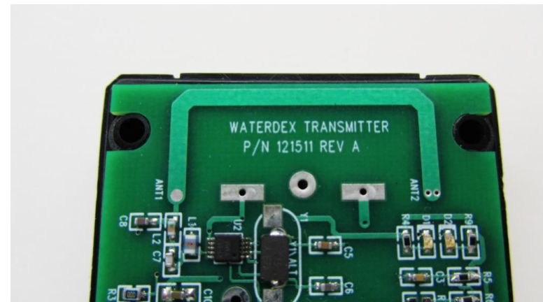
WD Transmitter \frac{1}{4} Wave Loop Antenna
