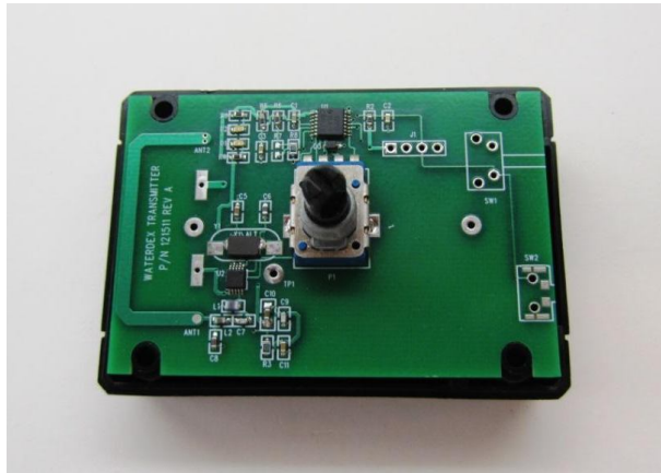
WD Transmitter PCB Front 1
