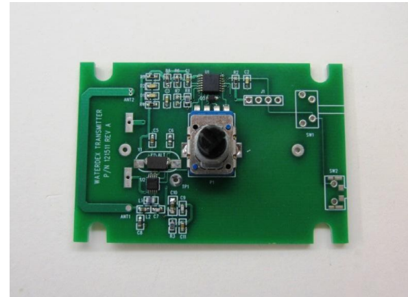
WD Transmitter PCB Front 2
