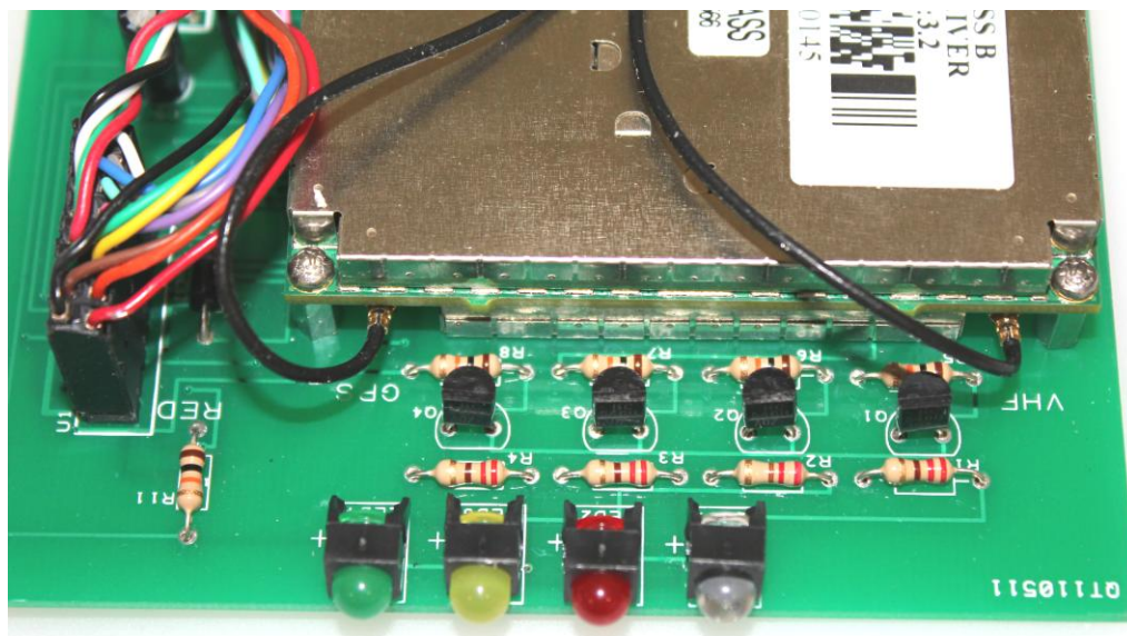
Figure 5 – LED Position-PCB
