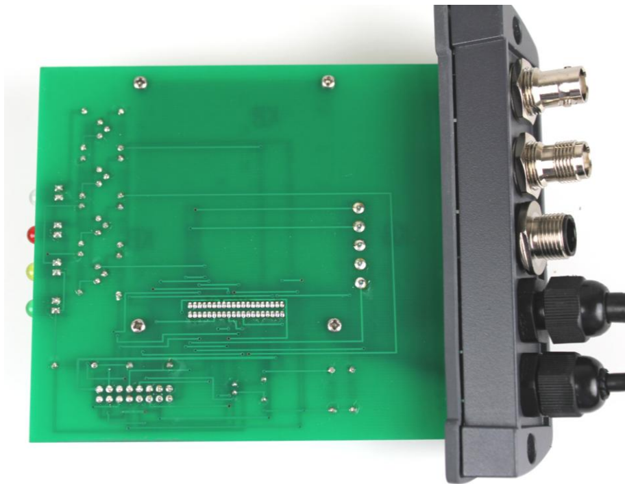
Figure 2 – Internal PCB -Bottom
