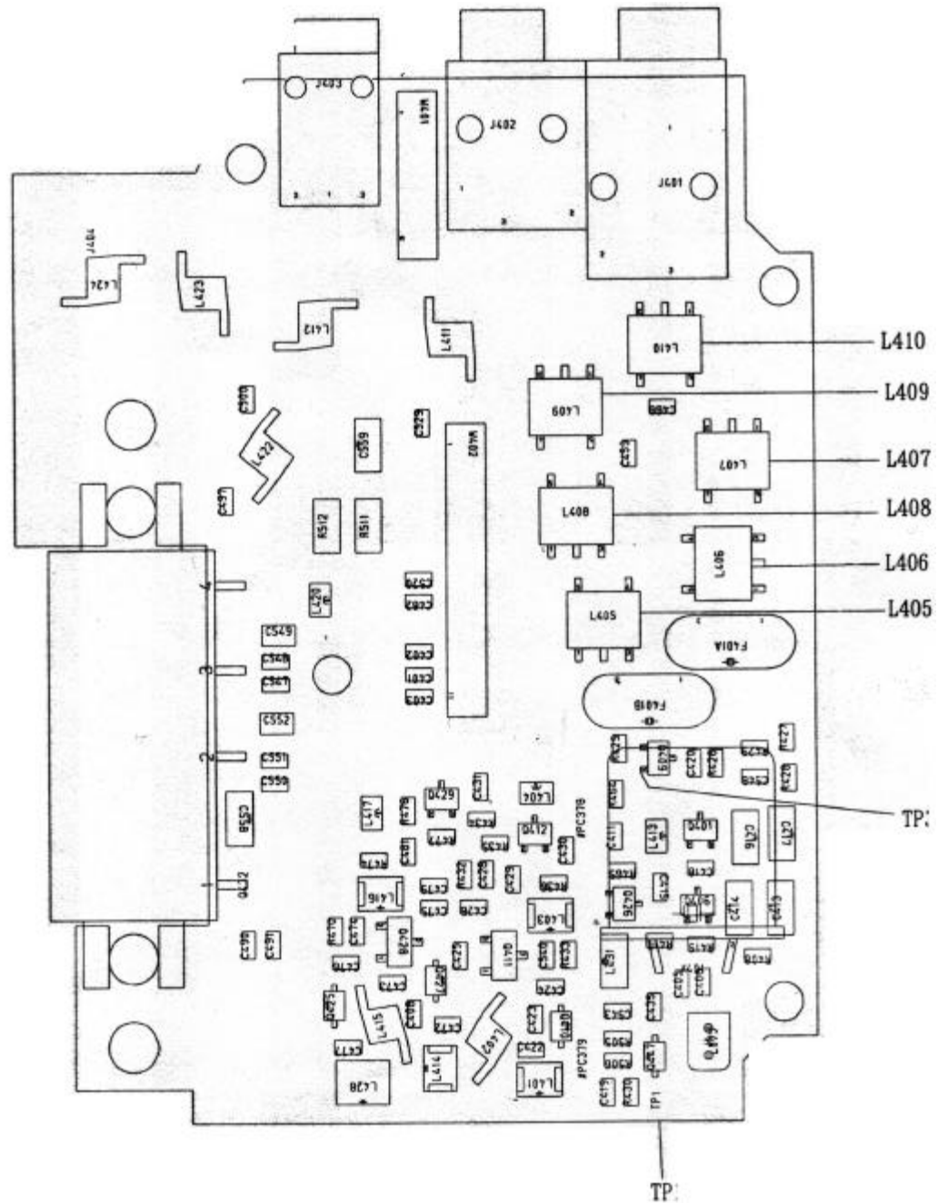
Componented Out RF Board op
