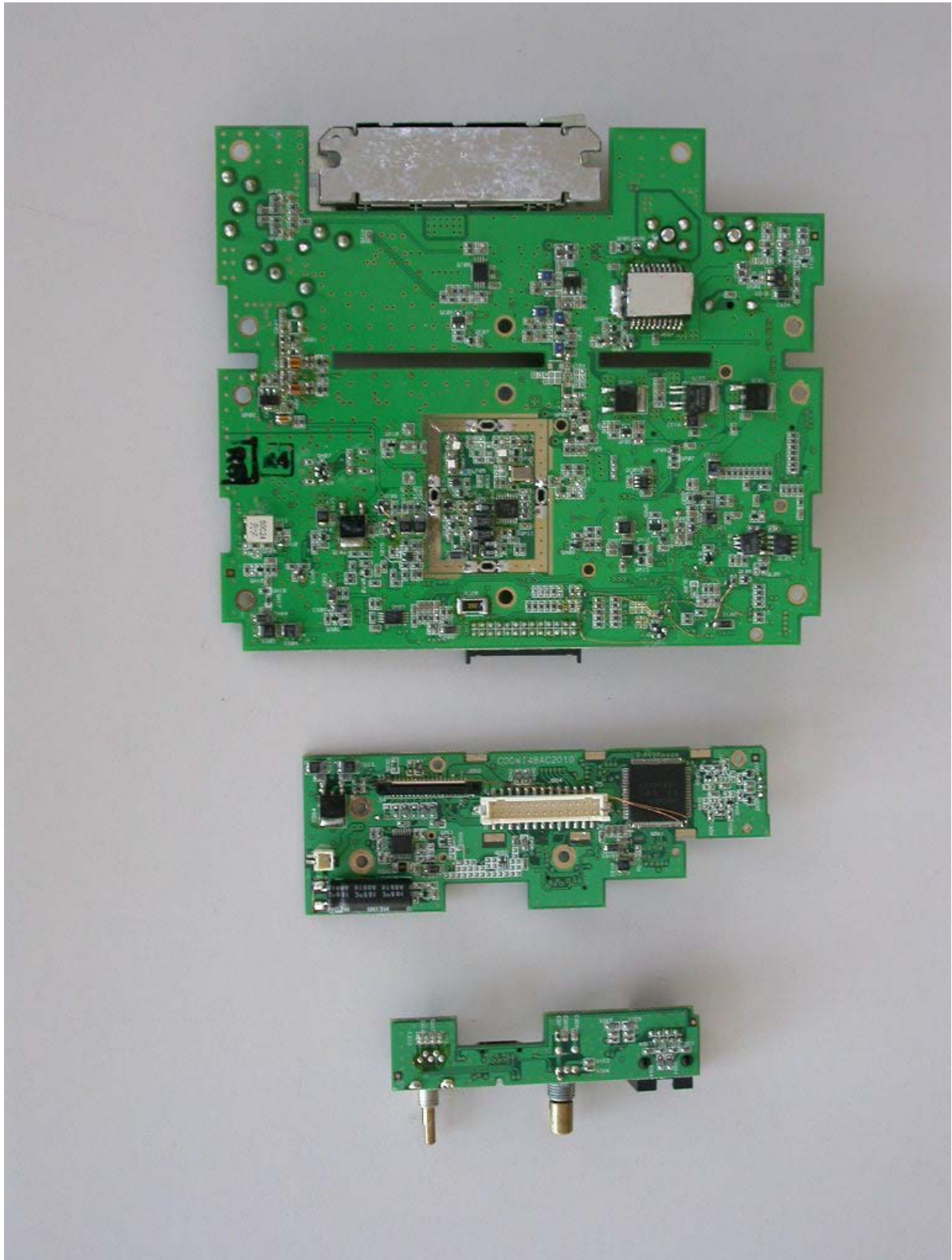
9) MAIN PCB of SC-980 (Solder Side View)
