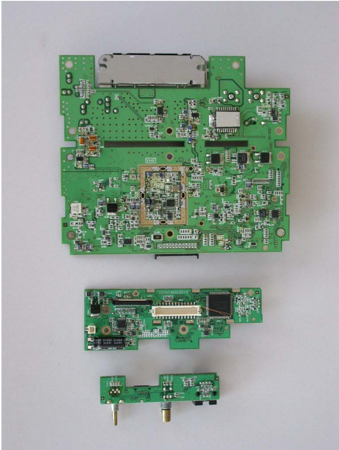
9) MAIN PCB of SC-780 (Solder Side View)
