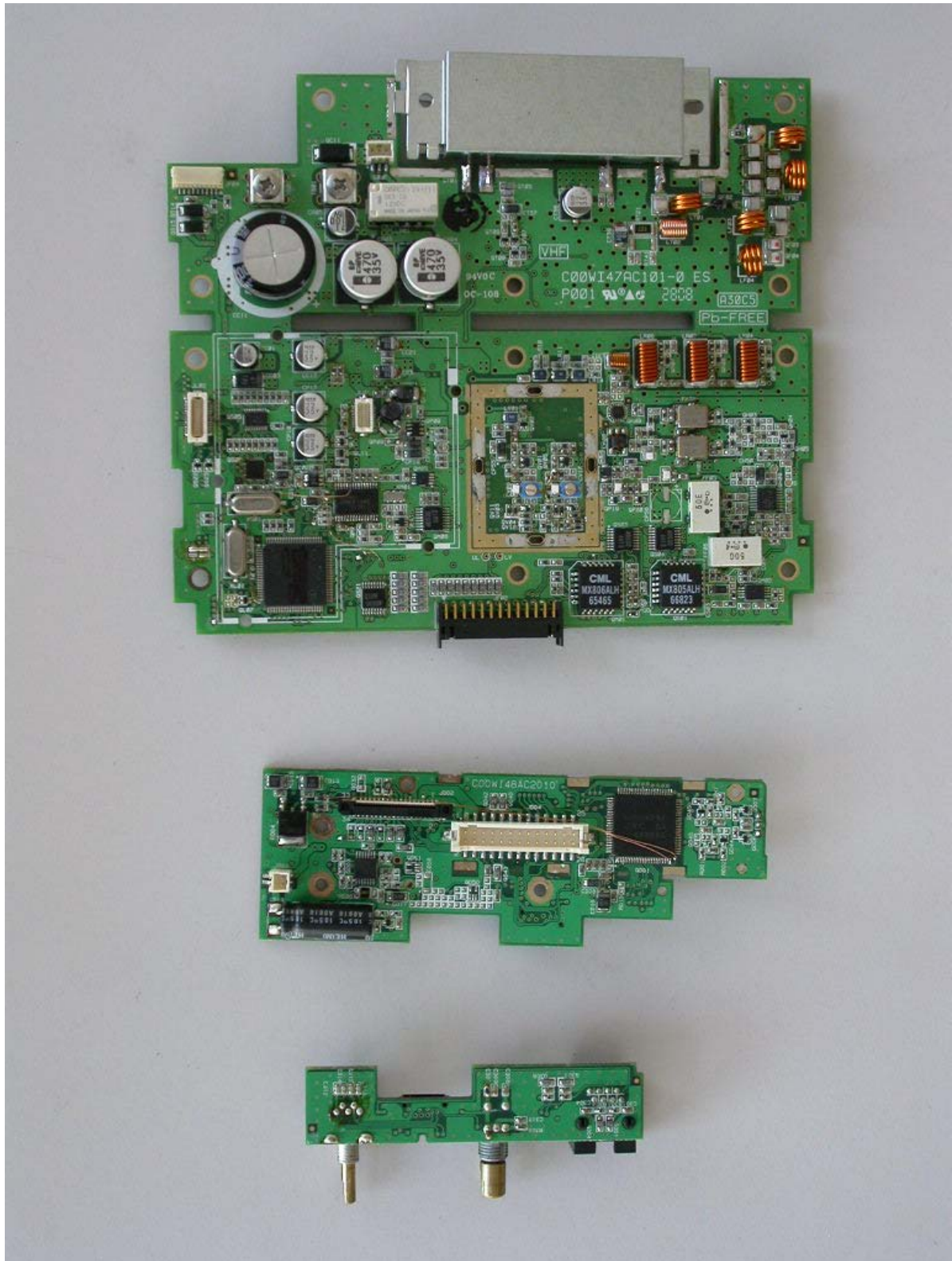
8) MAIN PCB of SC-780 (Component Side View)
