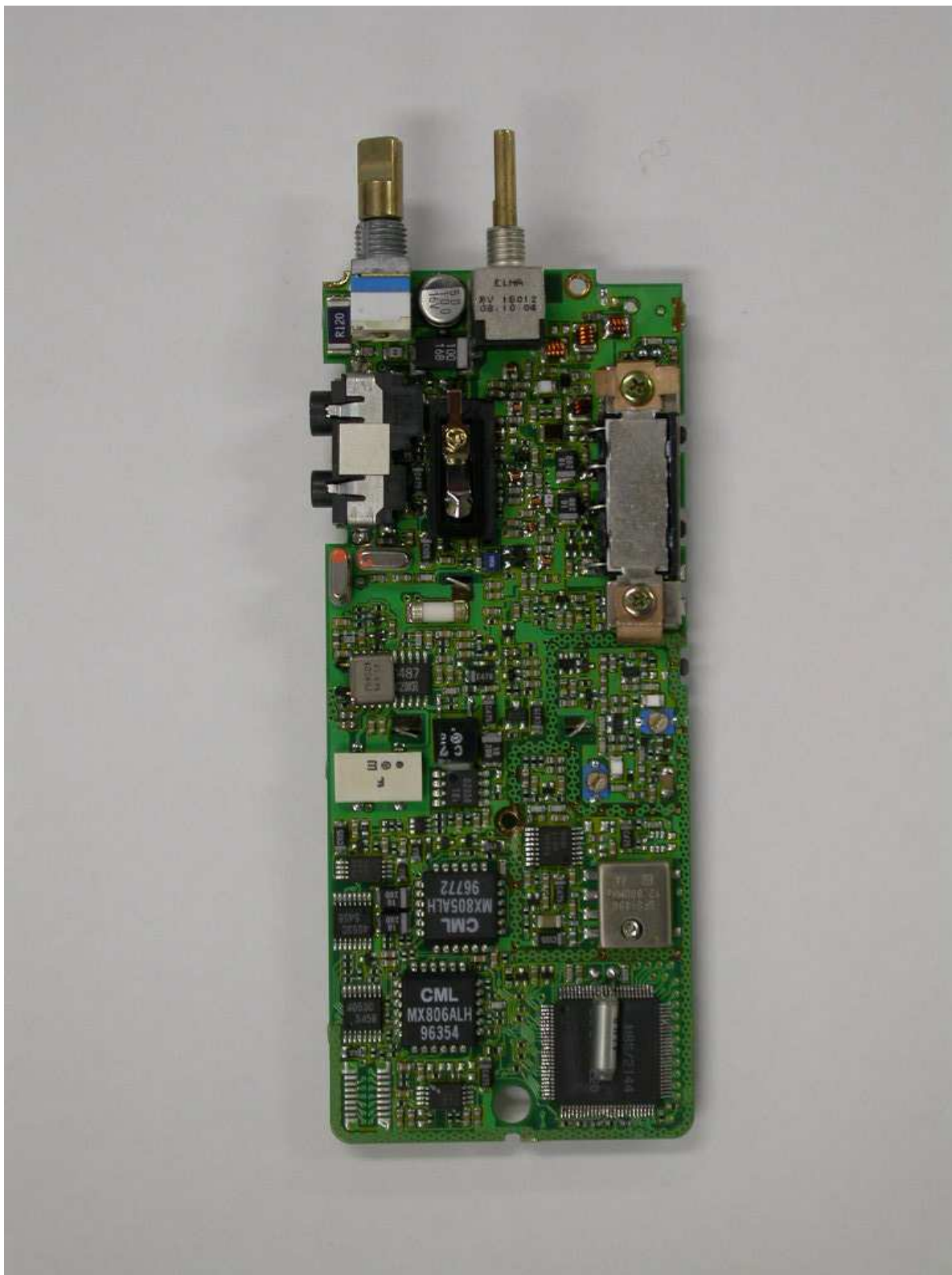
8) MAIN PCB of SC-580 (Solder Side View)
