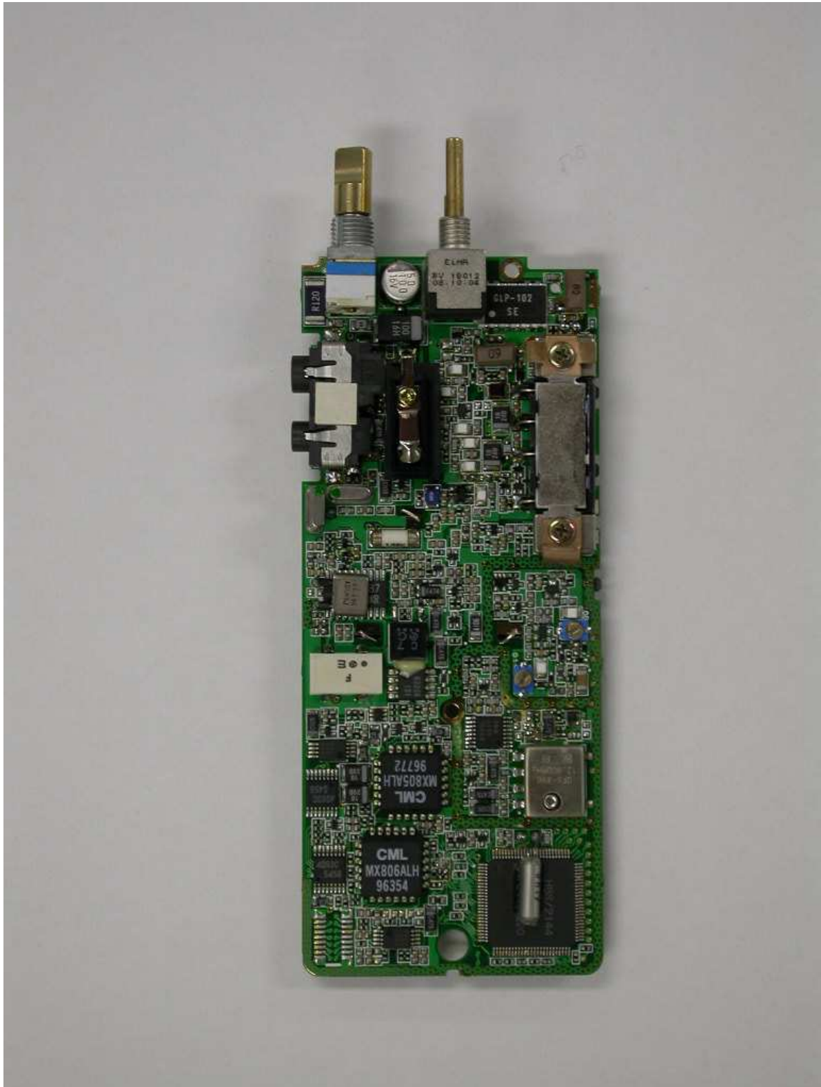
9) MAIN PCB of SC-280 (Solder Side View)
