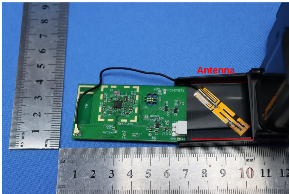
PIFA antenna version:
