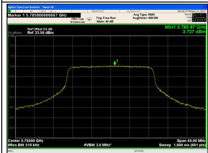
5725-5825MHz PSD - Mid CH 5785(White)
