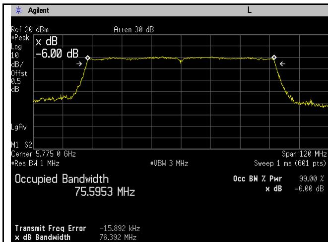
5725-5850MHz Bandwidth - One CH 5775 (Green)
