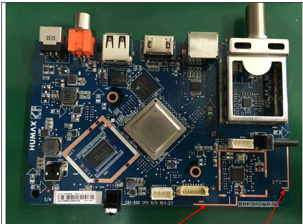
Antenna 1
