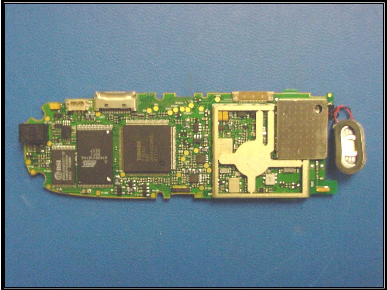
PHOTOGRAPH 19: PCB BACK WITH SHIELDS
