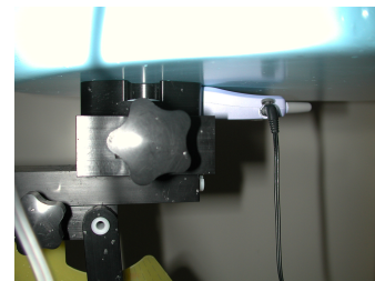
Figure 18. Body SAR Test Setup
