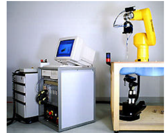
Fig. 1 SAR Test Setup
