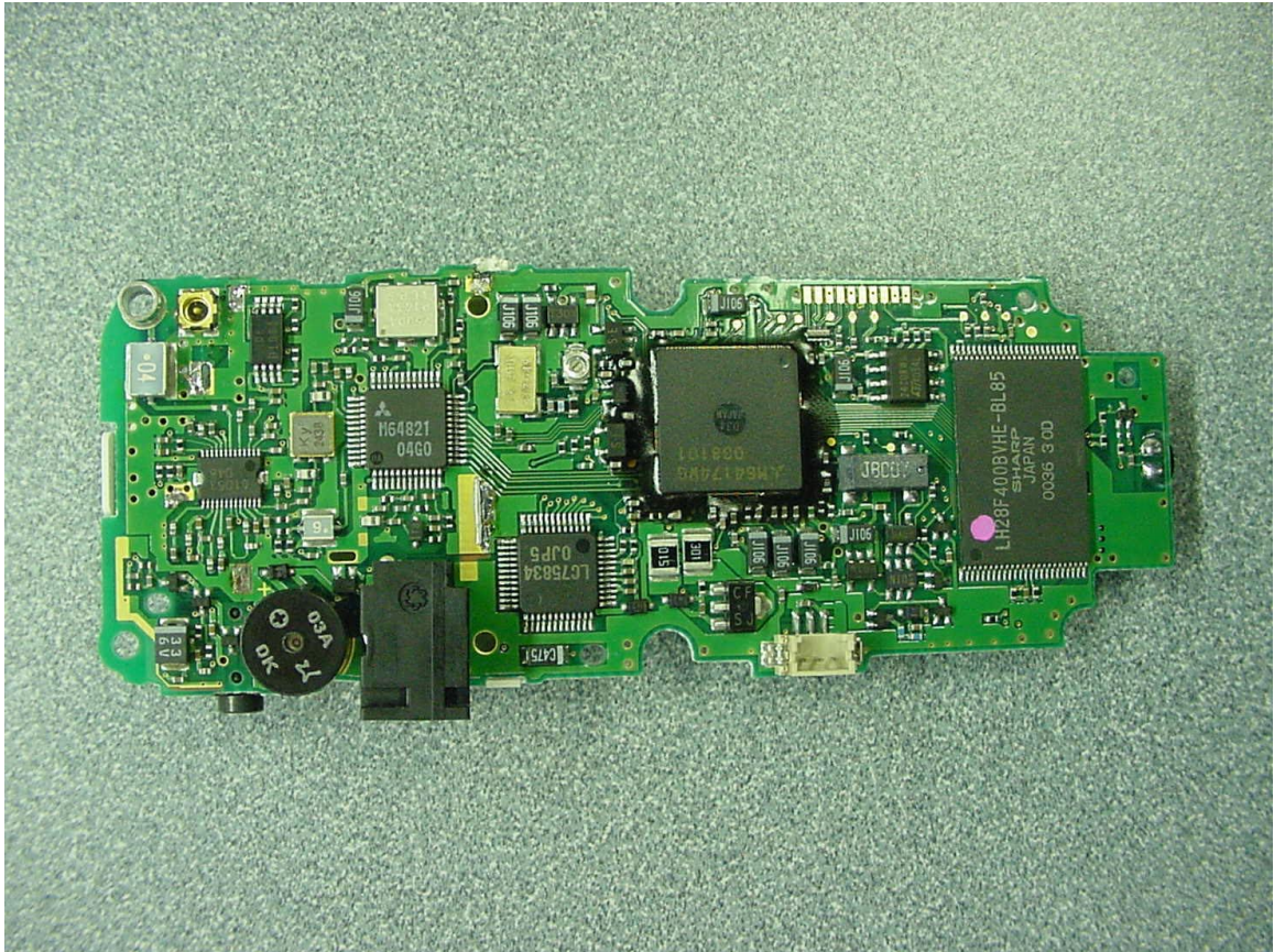
PHOTOGRAPH 23: BACK OF PCB WITH SHIELDS REMOVED
