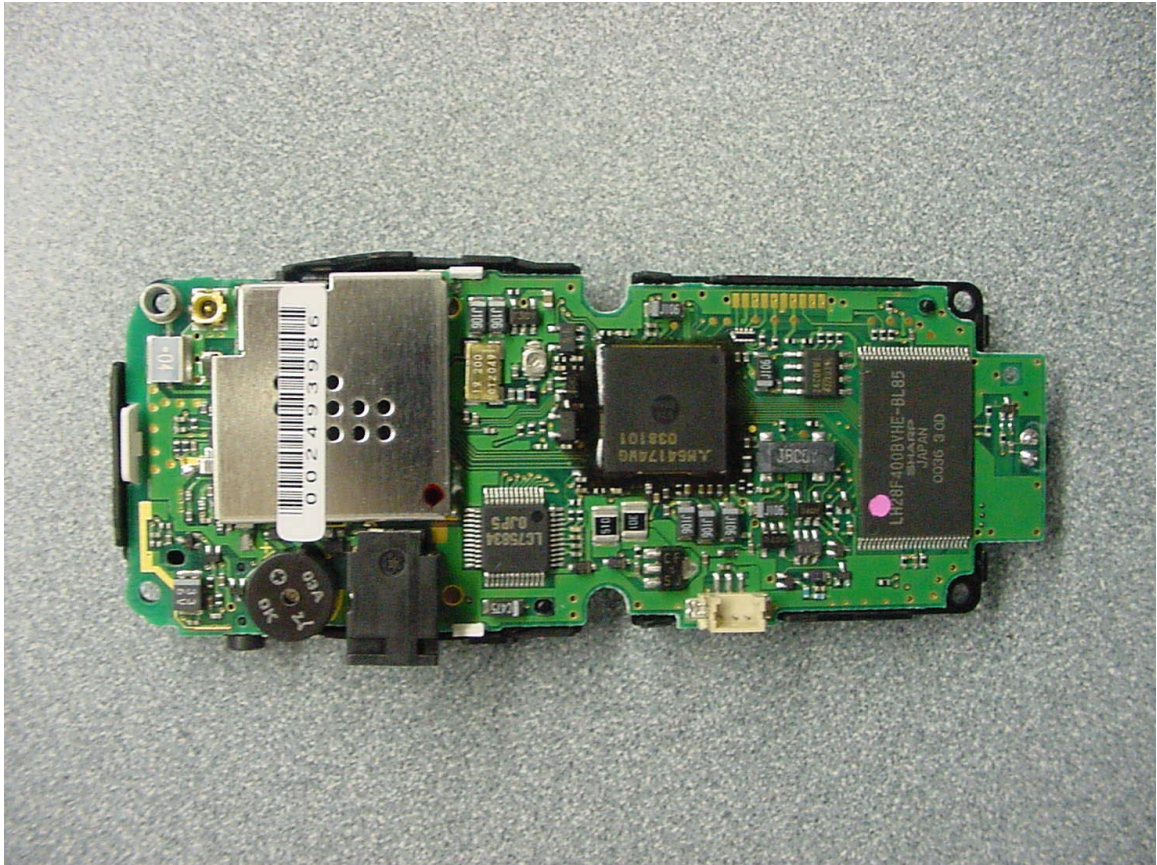
PHOTOGRAPH 22: BACK OF PCB WITH SHIELDS
