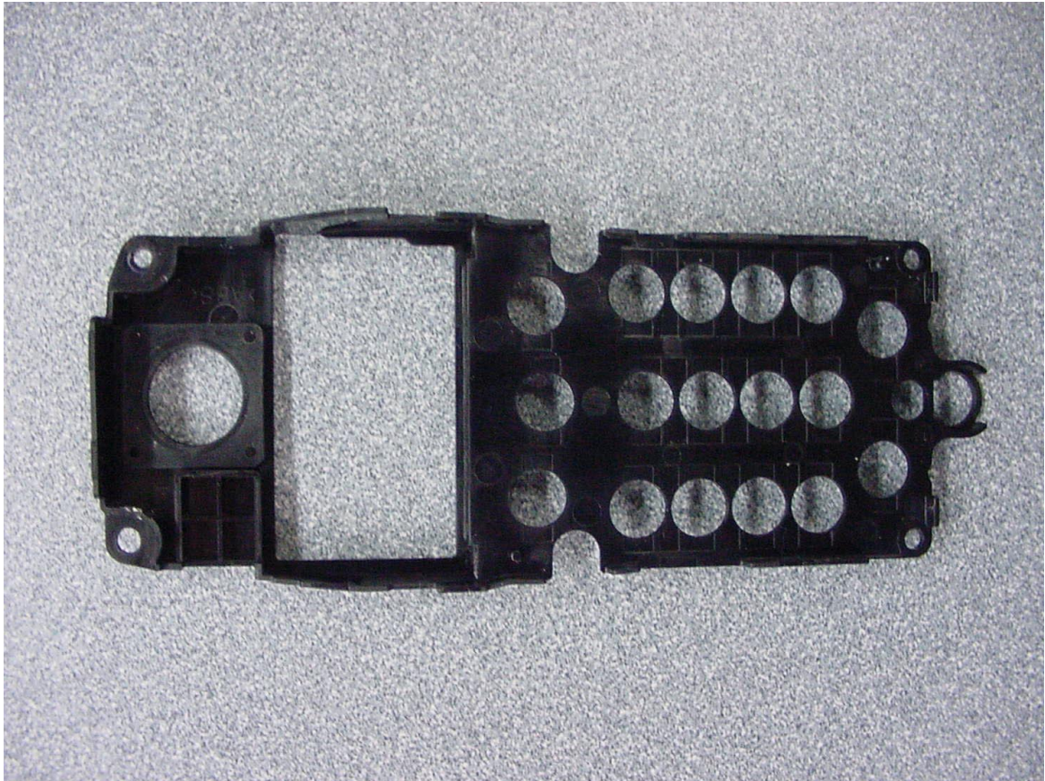
PHOTOGRAPH 17: BACK OF PLASTIC HOLDDOWN
