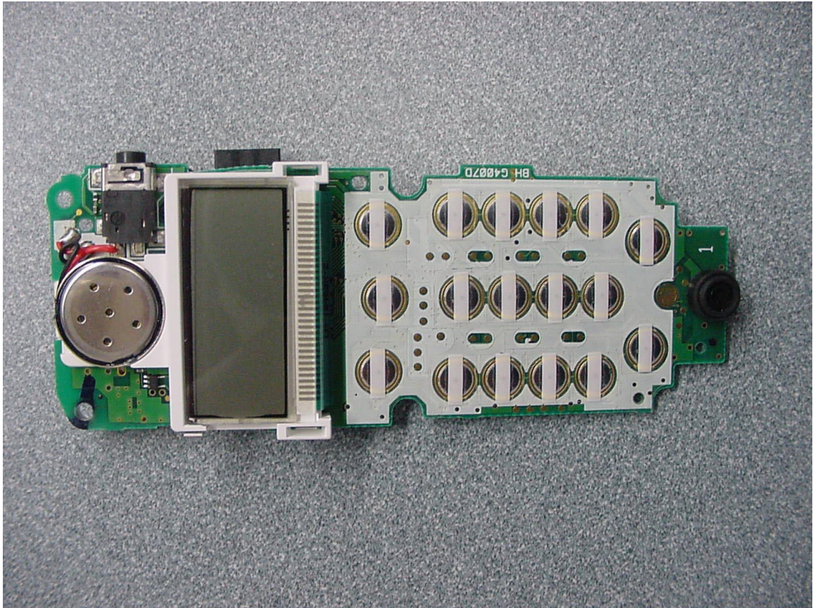
PHOTOGRAPH 20: FRONT OF PCB
