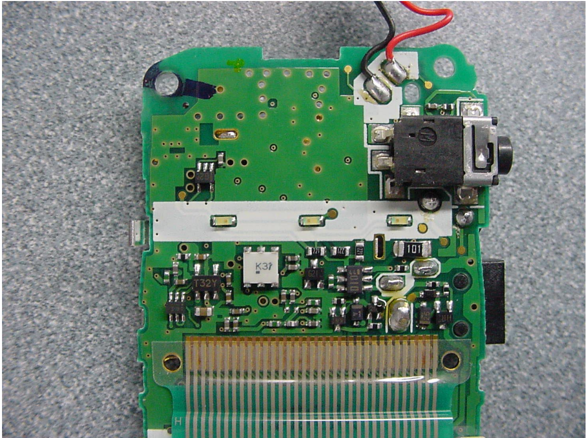
PHOTOGRAPH 21: UNDER LCD/SPEAKER ASSEMBLY (UPPER FRONT PCB)
