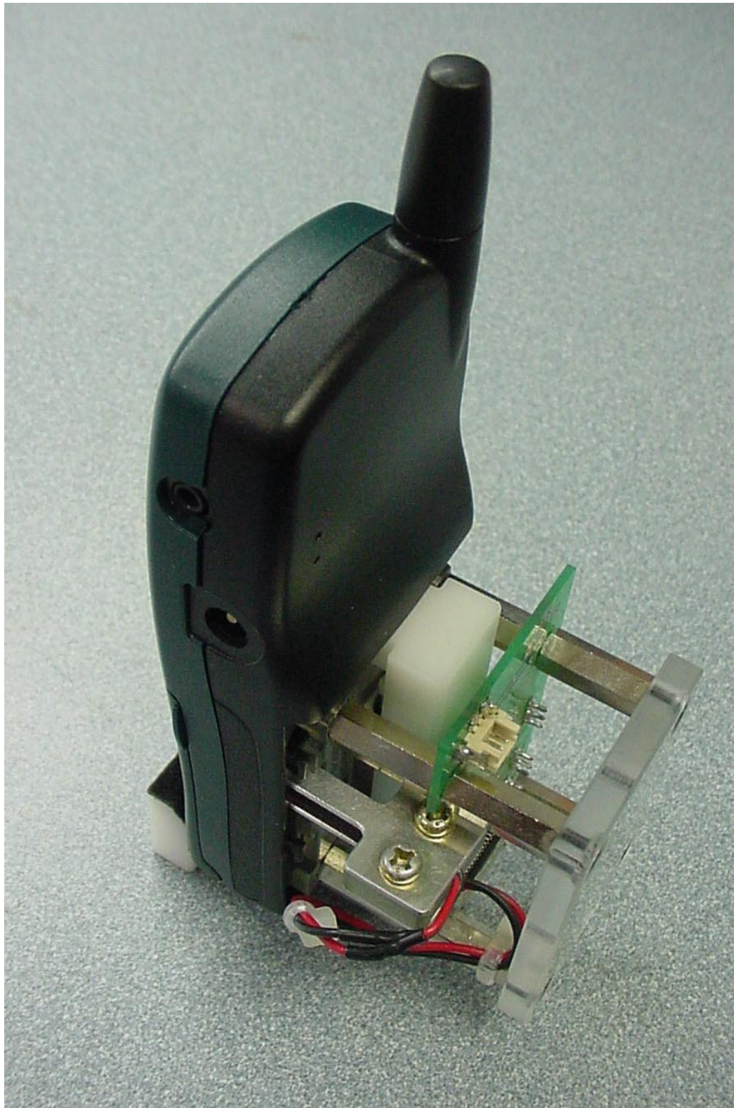
PHOTOGRAPH 35: TEST JIG MOUNTED TO PHONE
