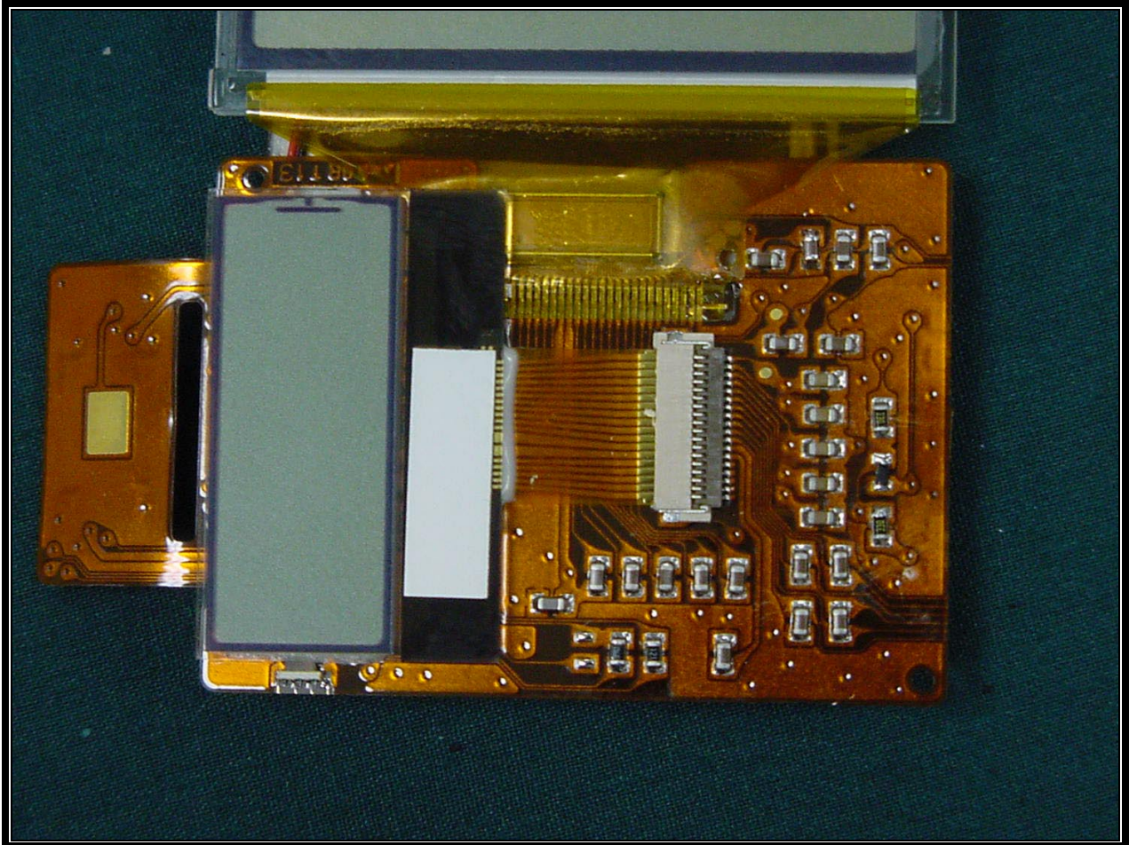
PHOTOGRAPH 25: LCD FRONT A BOARD CABLE
