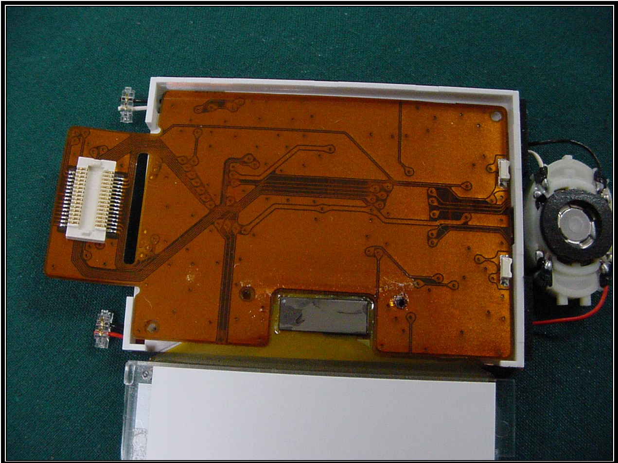
PHOTOGRAPH 27: BACK OF LCD BOARD CABLE
