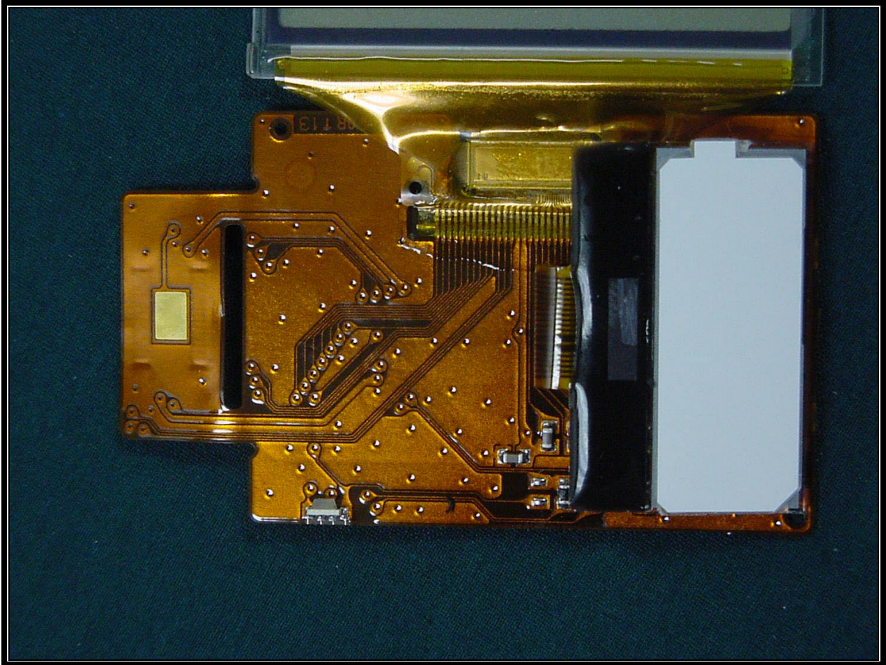
PHOTOGRAPH 26: LCD FRONT B BOARD CABLE
