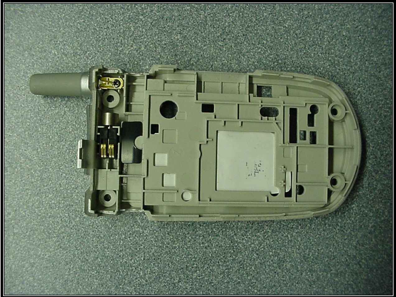
PHOTOGRAPH 32: INSIDE BATTERY BEZEL
