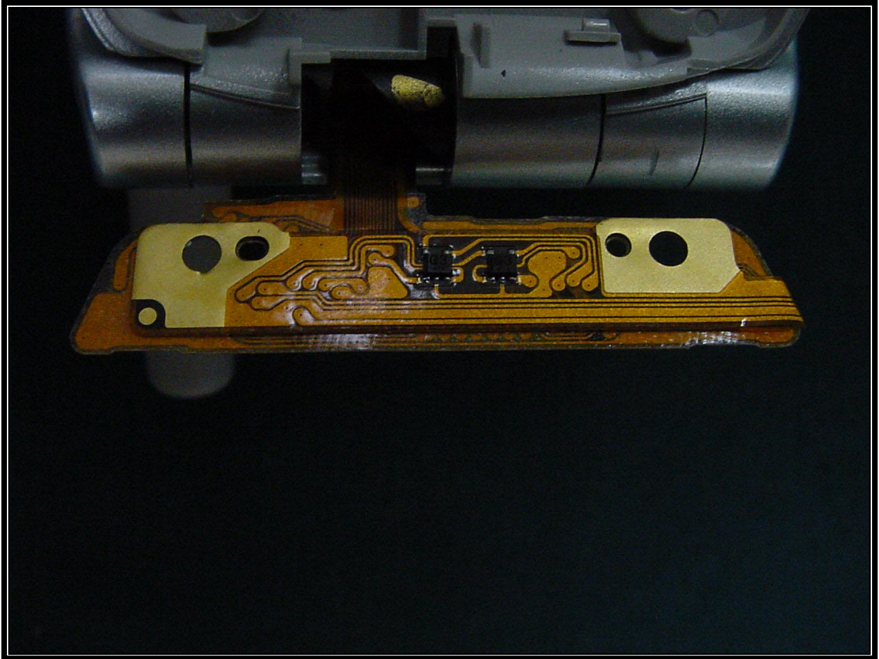
PHOTOGRAPH 29: BACK OF LCD CABLE
