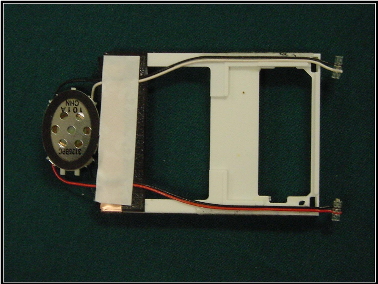
PHOTOGRAPH 21: LCD CHASSIS FRONT
