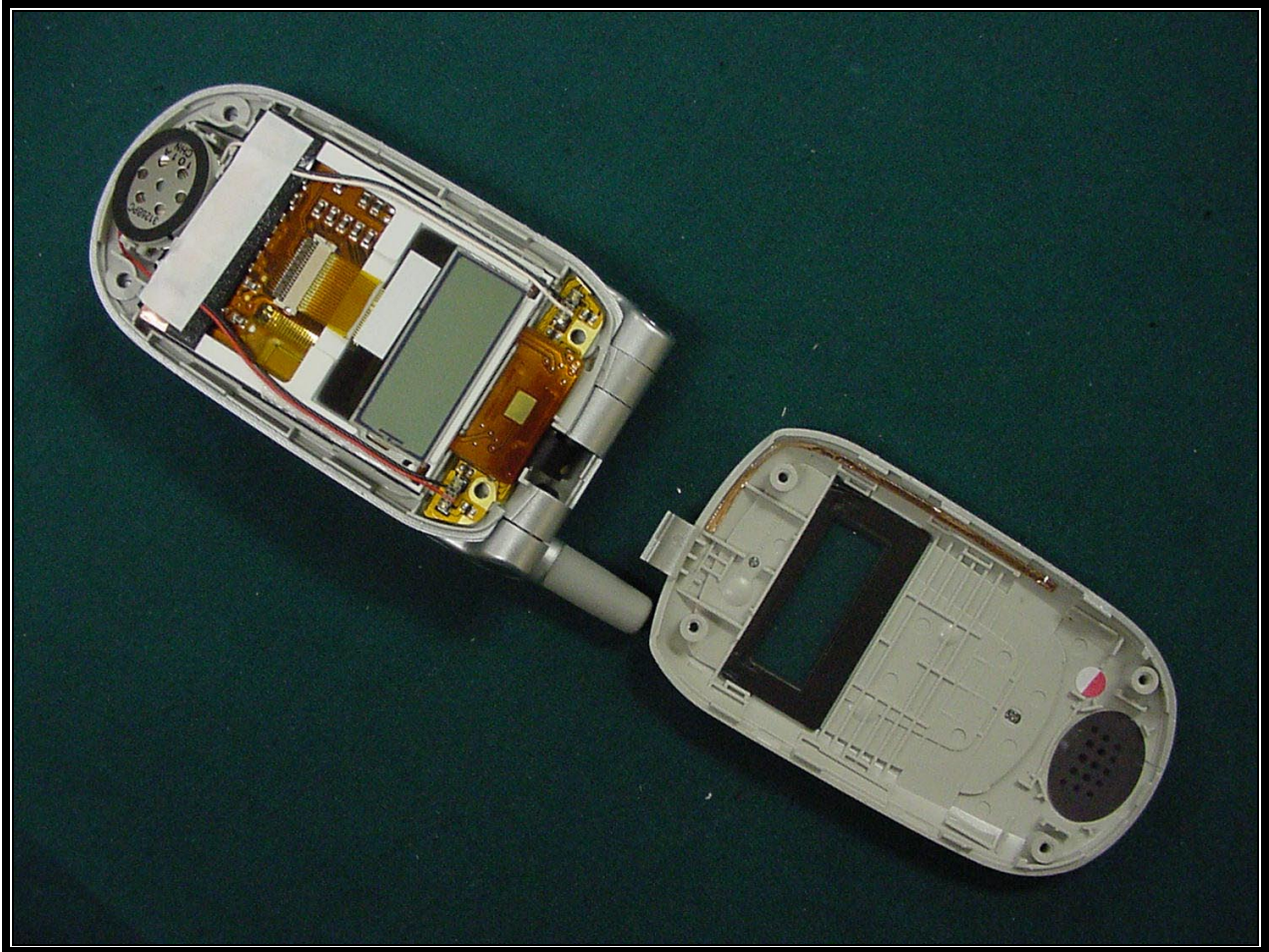
PHOTOGRAPH 15: INSIDE LCD ASSEMBLY
