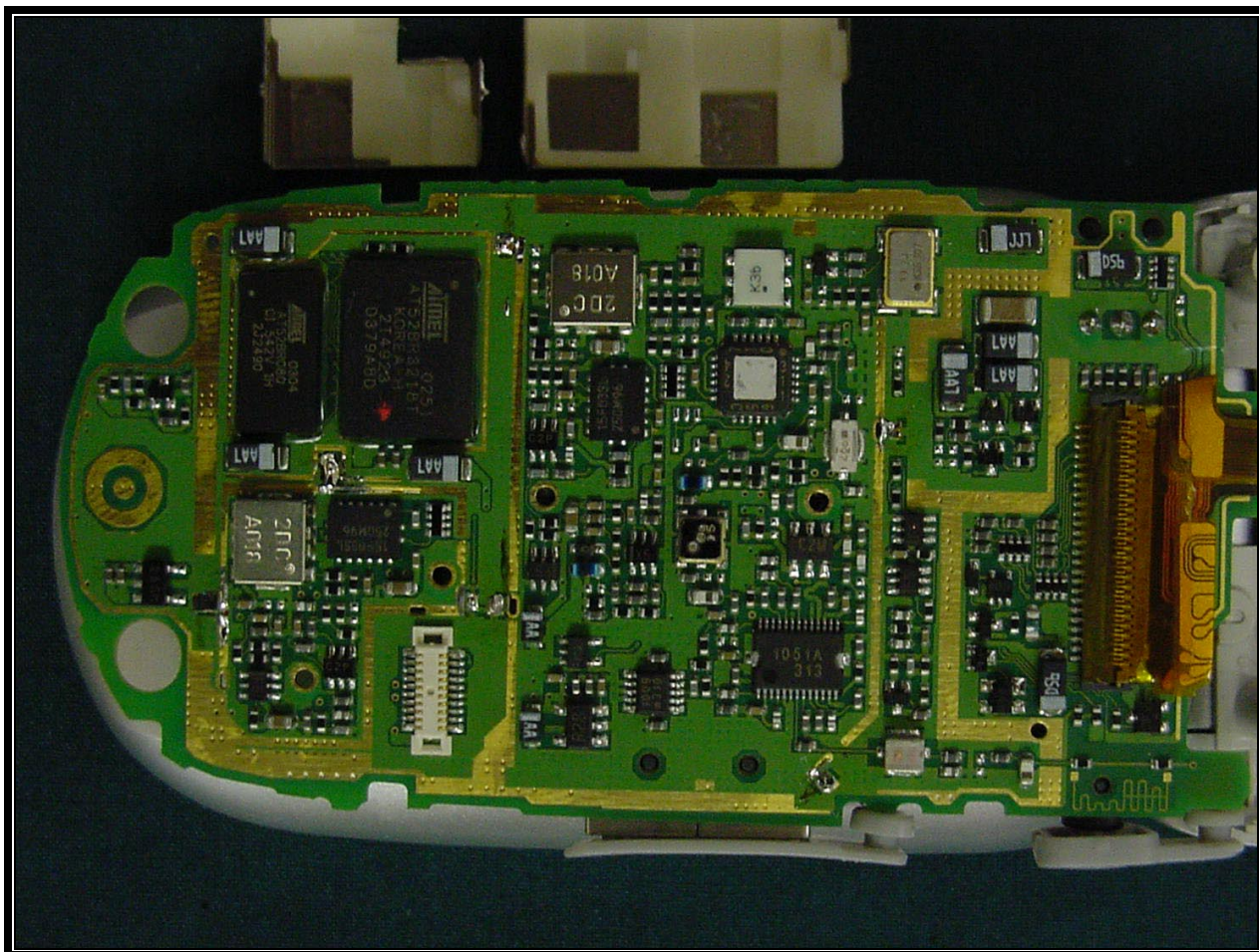
PHOTOGRAPH 20: BACK OF PCB WITHOUT SHIELDS
