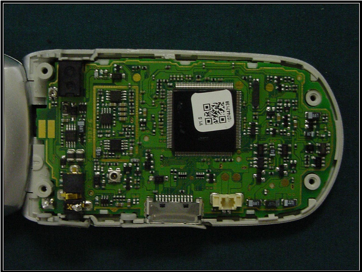
PHOTOGRAPH 18: FRONT OF PCB
