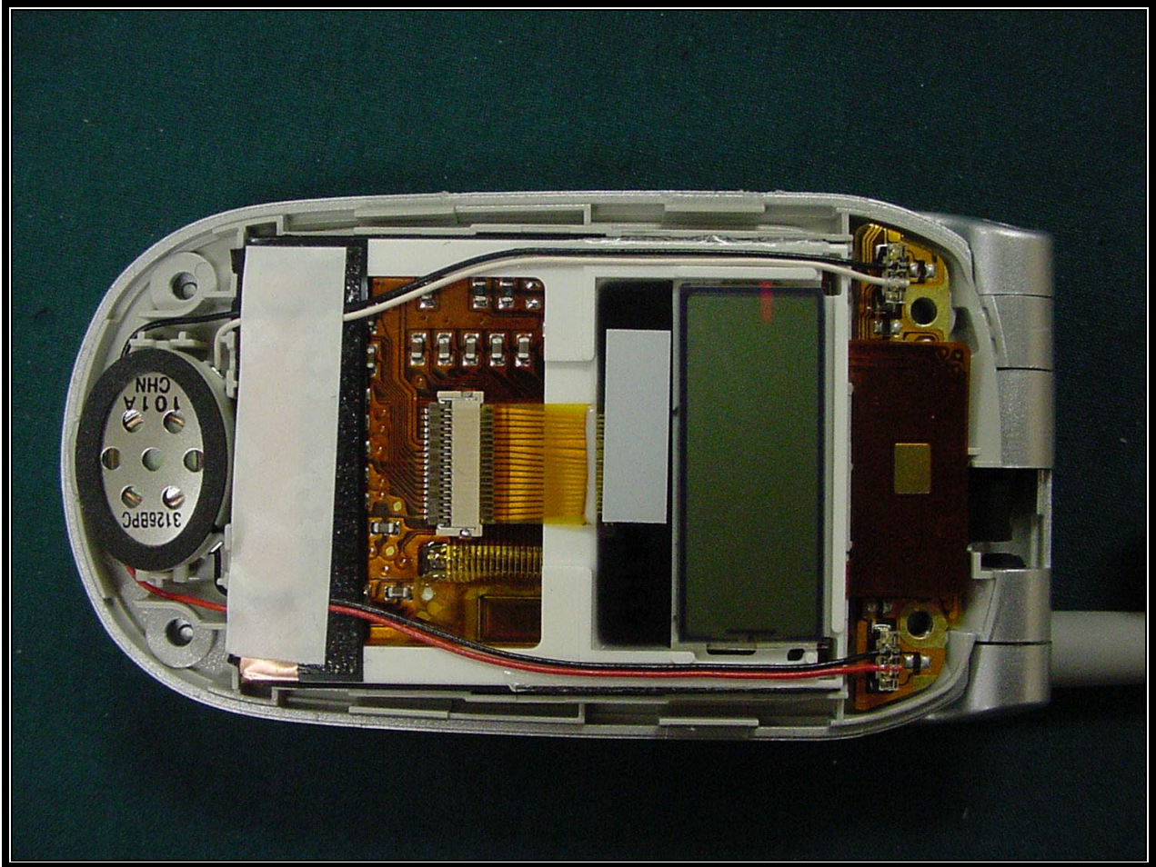
PHOTOGRAPH 23: BACK OF LCD ASSEMBLY
