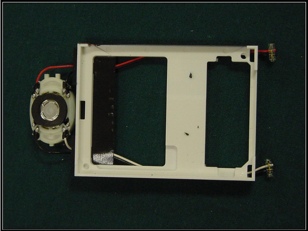
PHOTOGRAPH 22: LCD CHASSIS BACK
