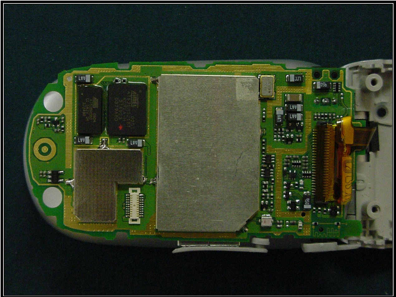
PHOTOGRAPH 19: BACK OF PCB WITH SHIELDS
