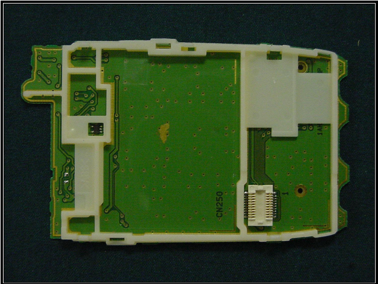
PHOTOGRAPH 17: BACK OF KEYPAD
