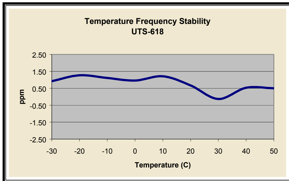
PLOT 9-1: TEMPERATURE FREQUENCY STABILITY - §2.1055
