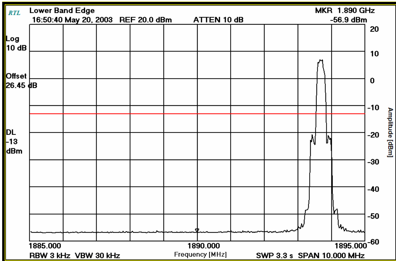
PLOT 8-1: LOWER BAND EDGE (LOWER BLOCK F)
