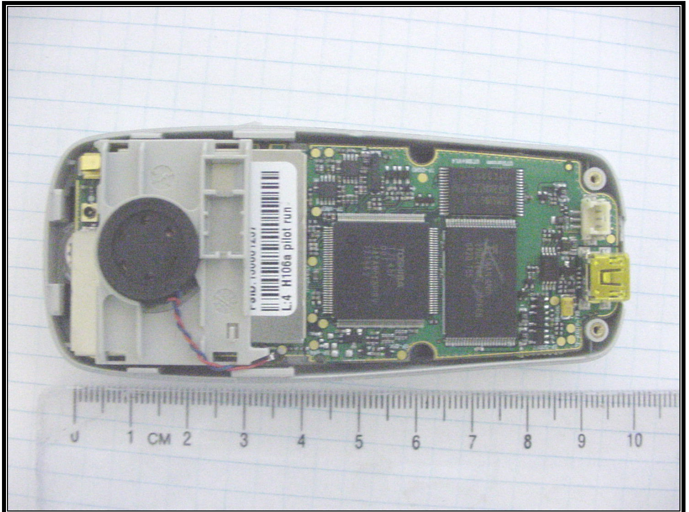
PHOTOGRAPH 13: PCB IN BACK COVER
