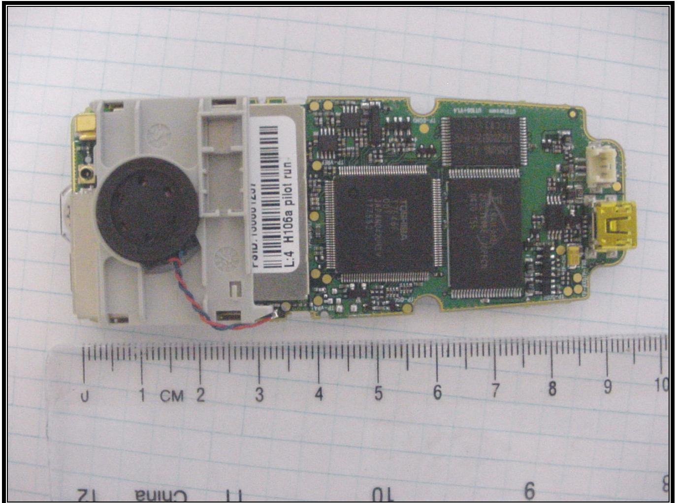
PHOTOGRAPH 14: BACK OF PCB WITH SPEAKER
