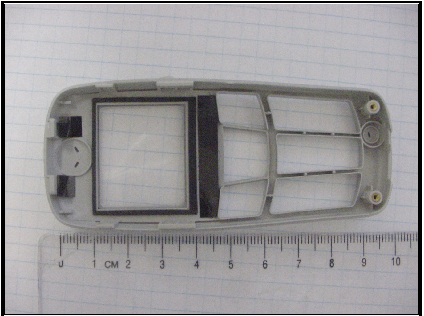
PHOTOGRAPH 12: INSIDE FRONT COVER
