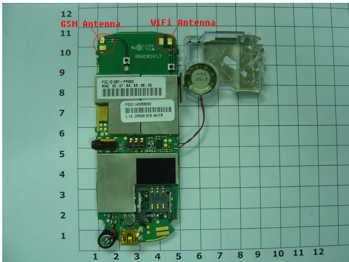
Antenna locations relative to chassis/housing
