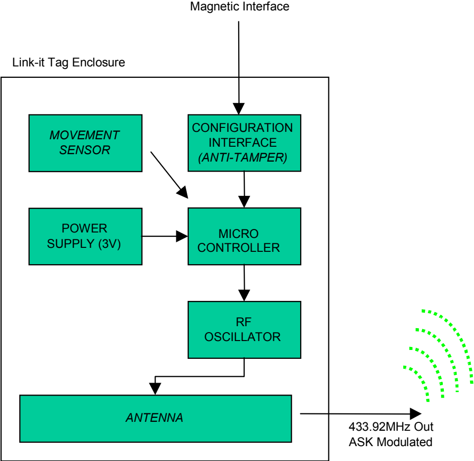
Block Diagram of the Tag L-TG800:
