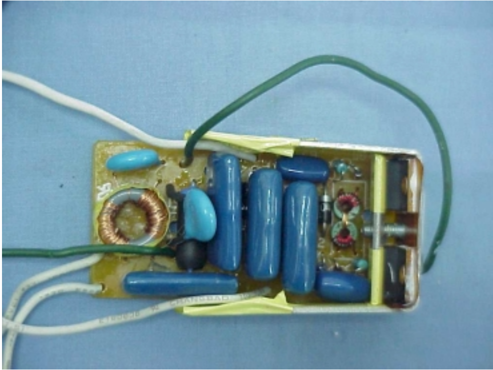
FIGURE 5. POWER SUPPLIES (M/N: 75W) MAIN BOARD (SOLDERED SIDE)
