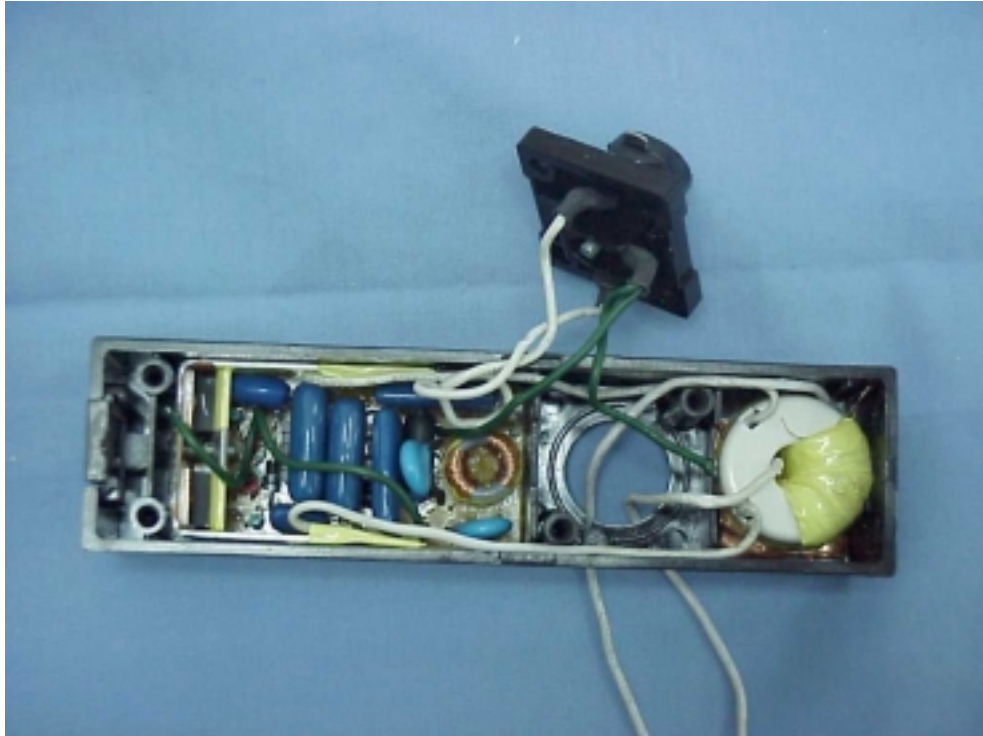
FIGURE 3. POWER SUPPLIES (M/N: 75W) INSIDE VIEW
