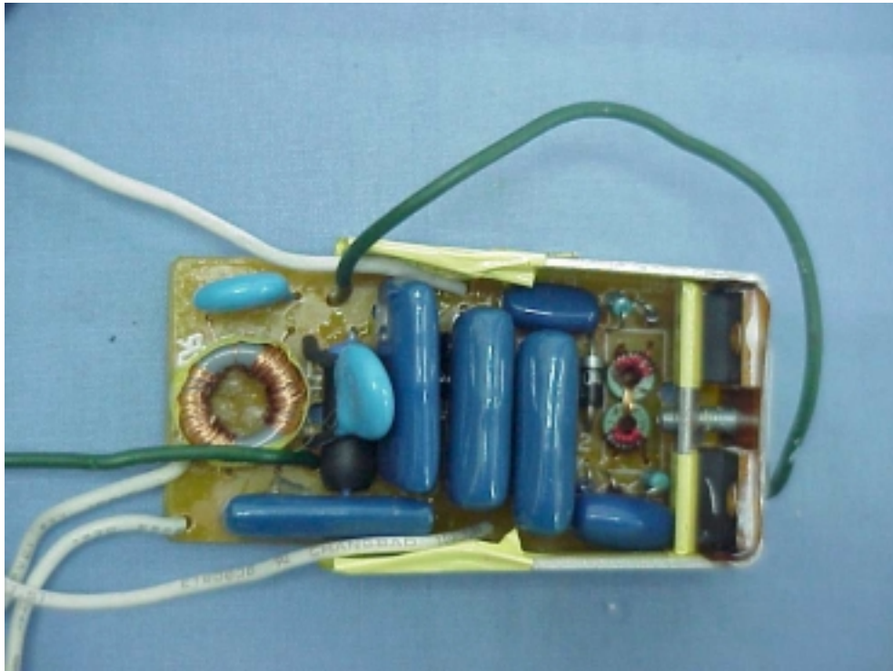
FIGURE 5. POWER SUPPLIES (M/N: 50W) MAIN BOARD (SOLDERED SIDE)
