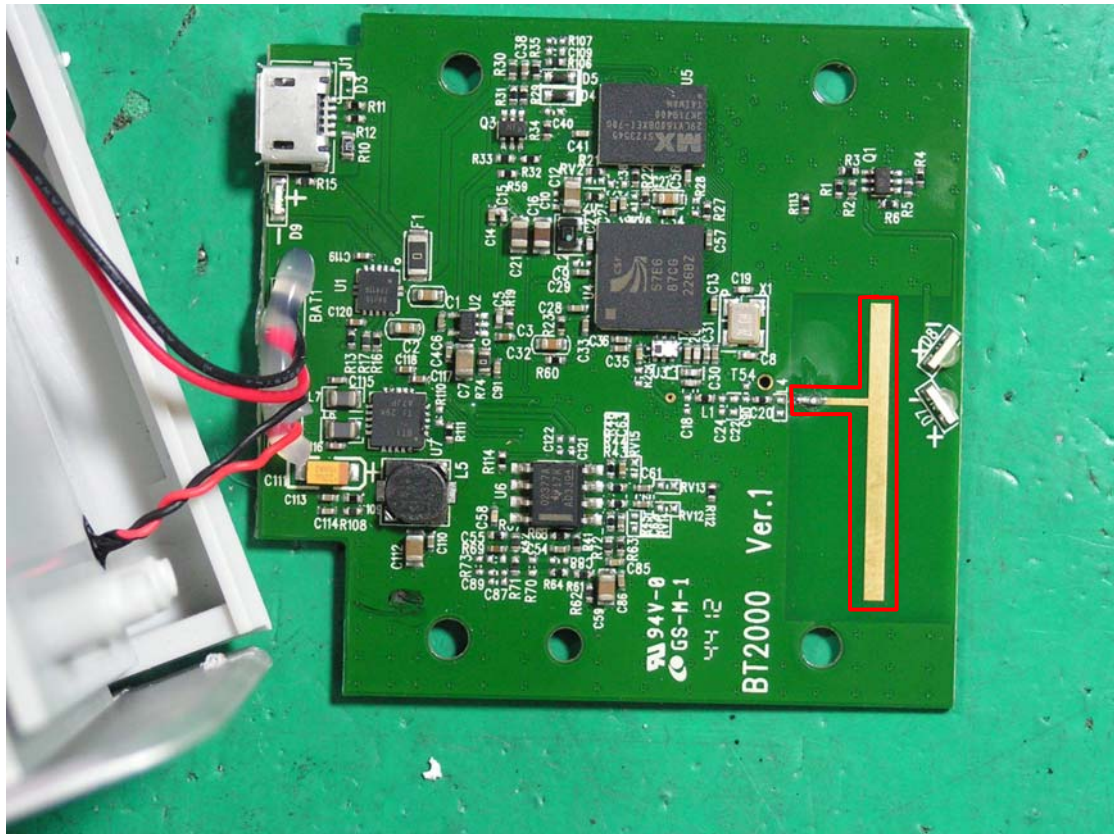
6. Antenna
