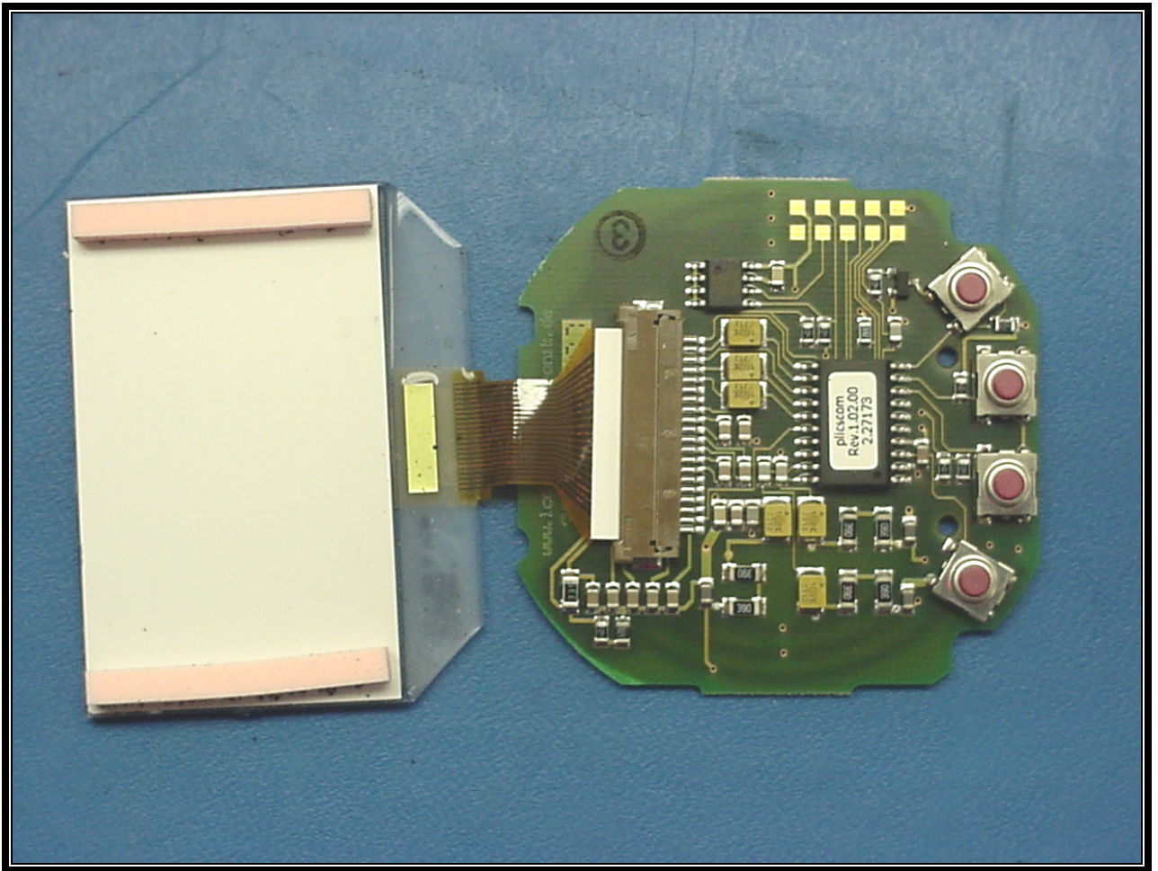
PHOTOGRAPH 22: EUT LCD DISPLAY – PCB TOP VIEW
