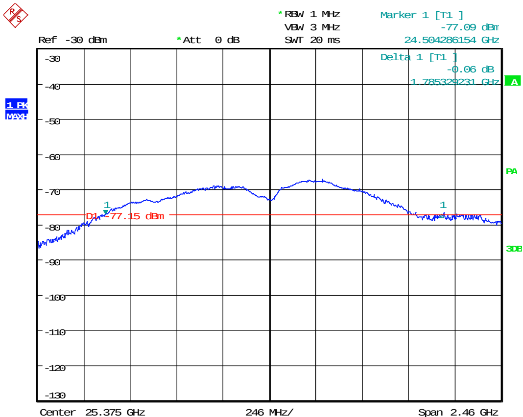
Plot 3-1: 10 dB Modulated Bandwidth
