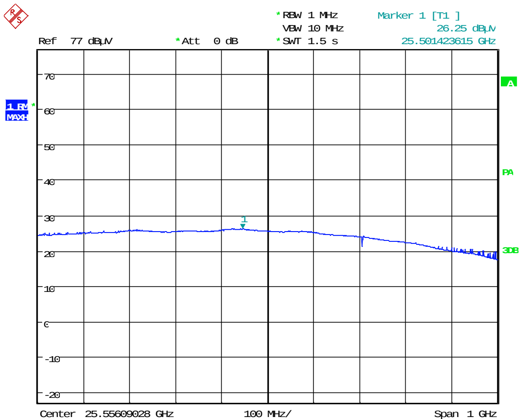
Plot 4-1: Radiated Fundamental (EIRP in 1 MHz)
