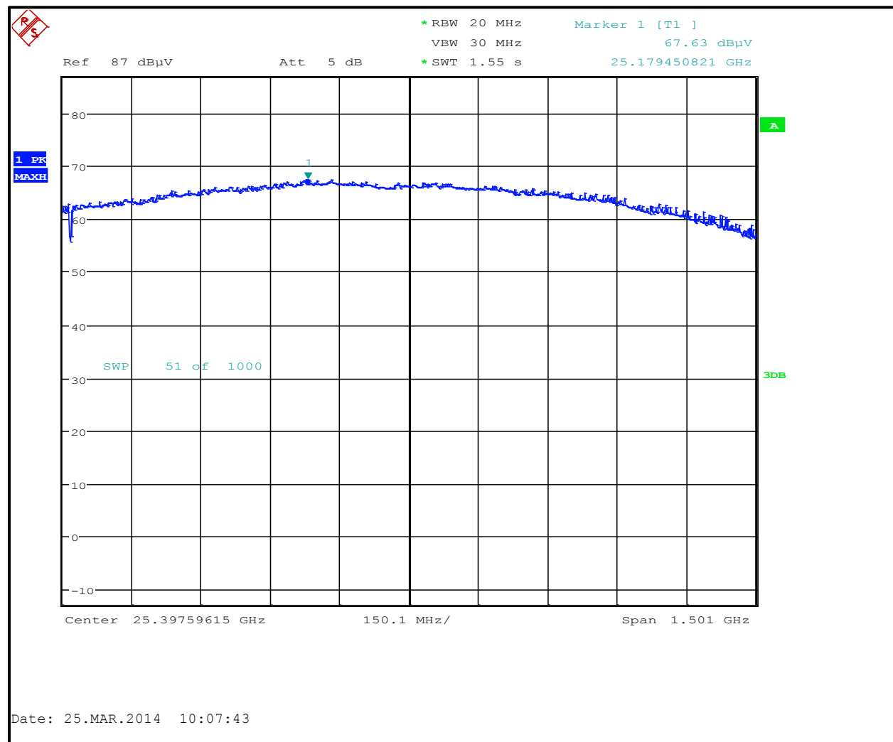
Plot 4-2: Radiated Fundamental (EIRP in 20 MHz)
