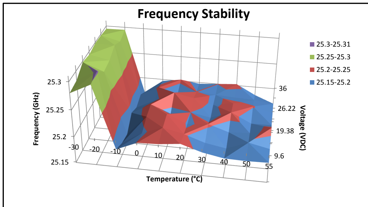
Plot 5-1: Frequency Stability – Voltage/Temperature/ppm
