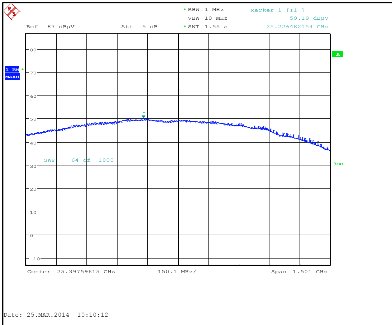
Plot 4-1: Radiated Fundamental (EIRP in 1 MHz)
