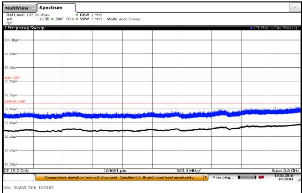
Plot 6-60: Radiated Emissions 12.4 GHz – 18 GHz; Fiberglass Container; TC #2, Horizontal
