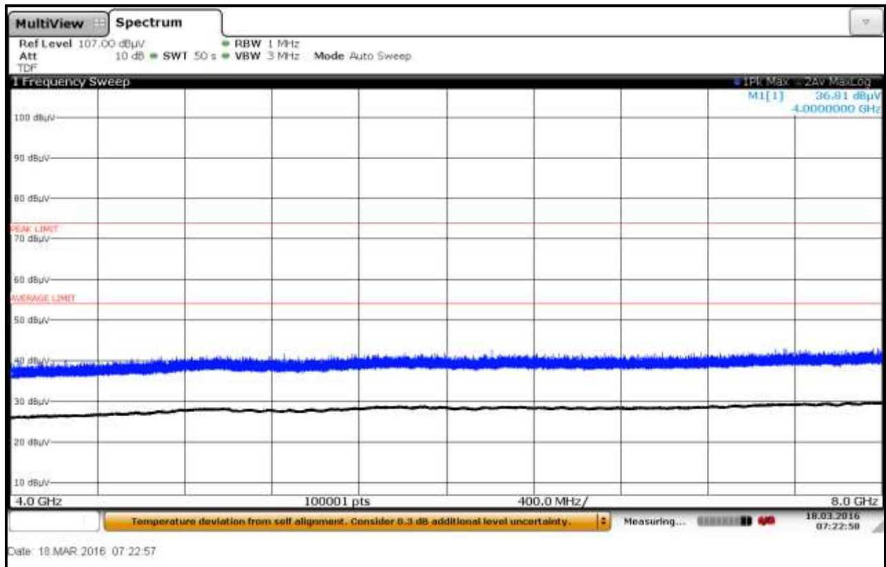
Plot 6-86: Radiated Emissions 4 GHz – 8 GHz; Fiberglass Container; TC #3; Horizontal
