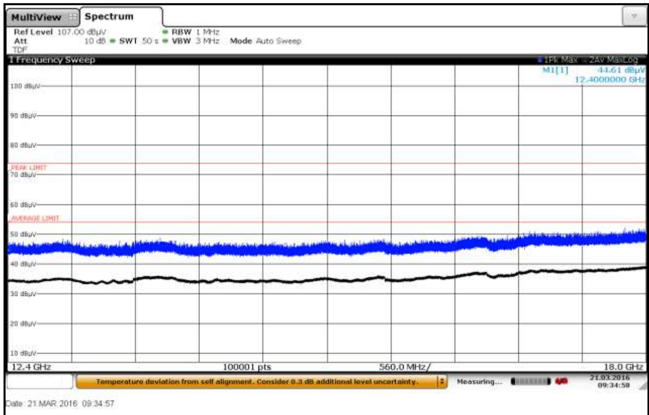
Plot 6-81: Radiated Emissions 12.4 GHz – 18 GHz; Concrete Container; TC #3, Vertical
