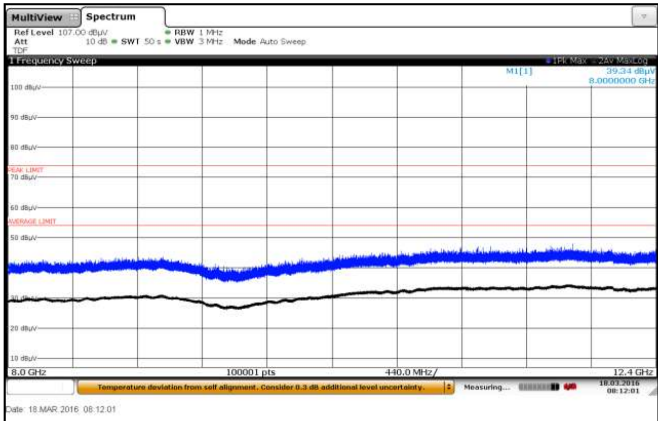
Plot 6-89: Radiated Emissions 8 GHz – 12.4 GHz; Fiberglass Container; TC #3, Vertical
