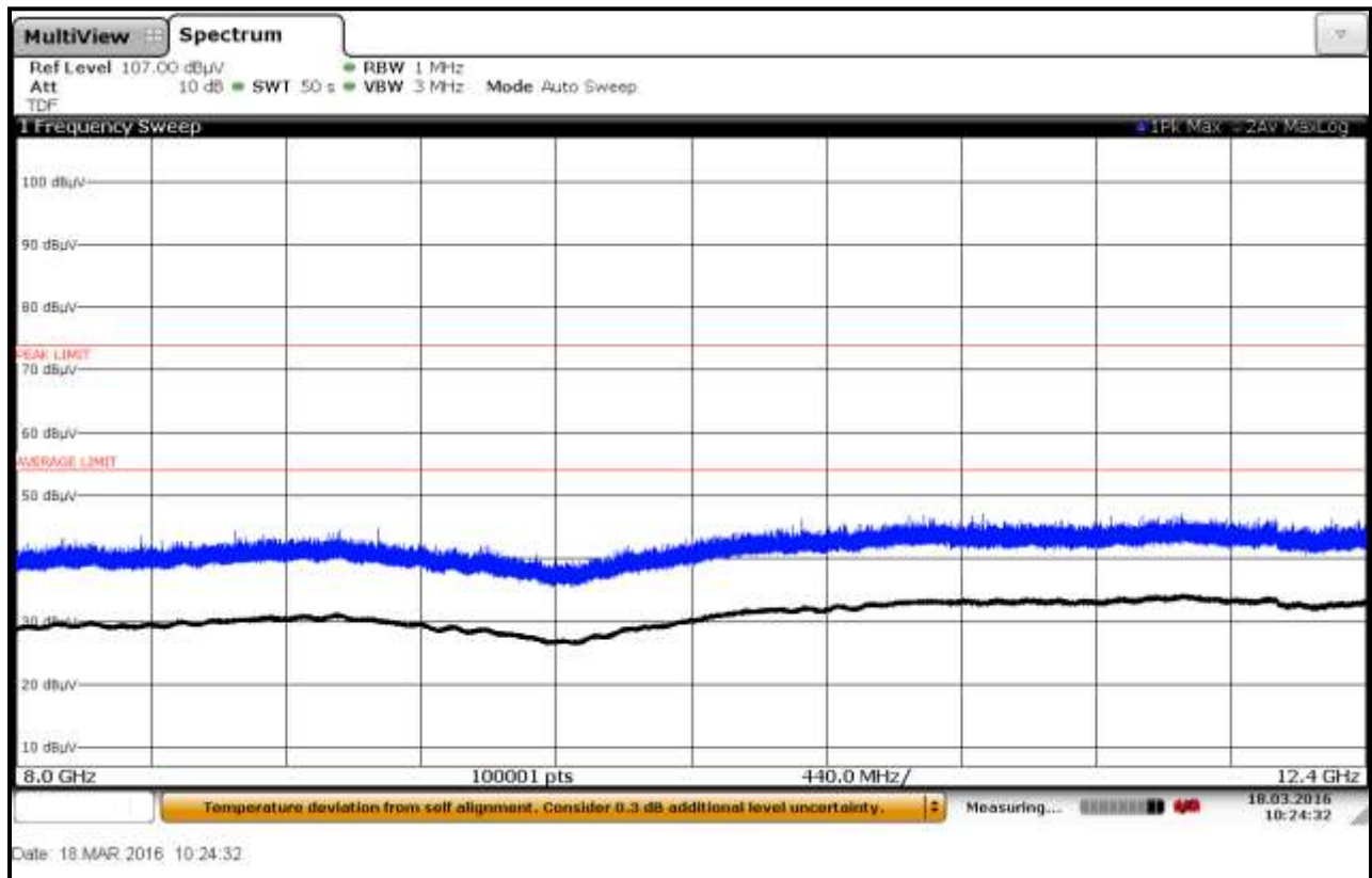
Plot 6-58: Radiated Emissions 8 GHz – 12.4 GHz; Fiberglass Container; TC #2, Horizontal
