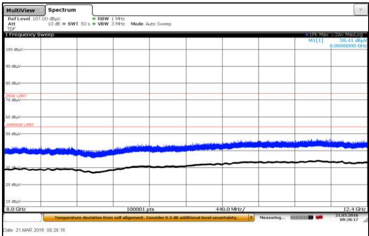
Plot 6-48: Radiated Emissions 8 GHz – 12.4 GHz; Concrete Container; TC #2, Horizontal
