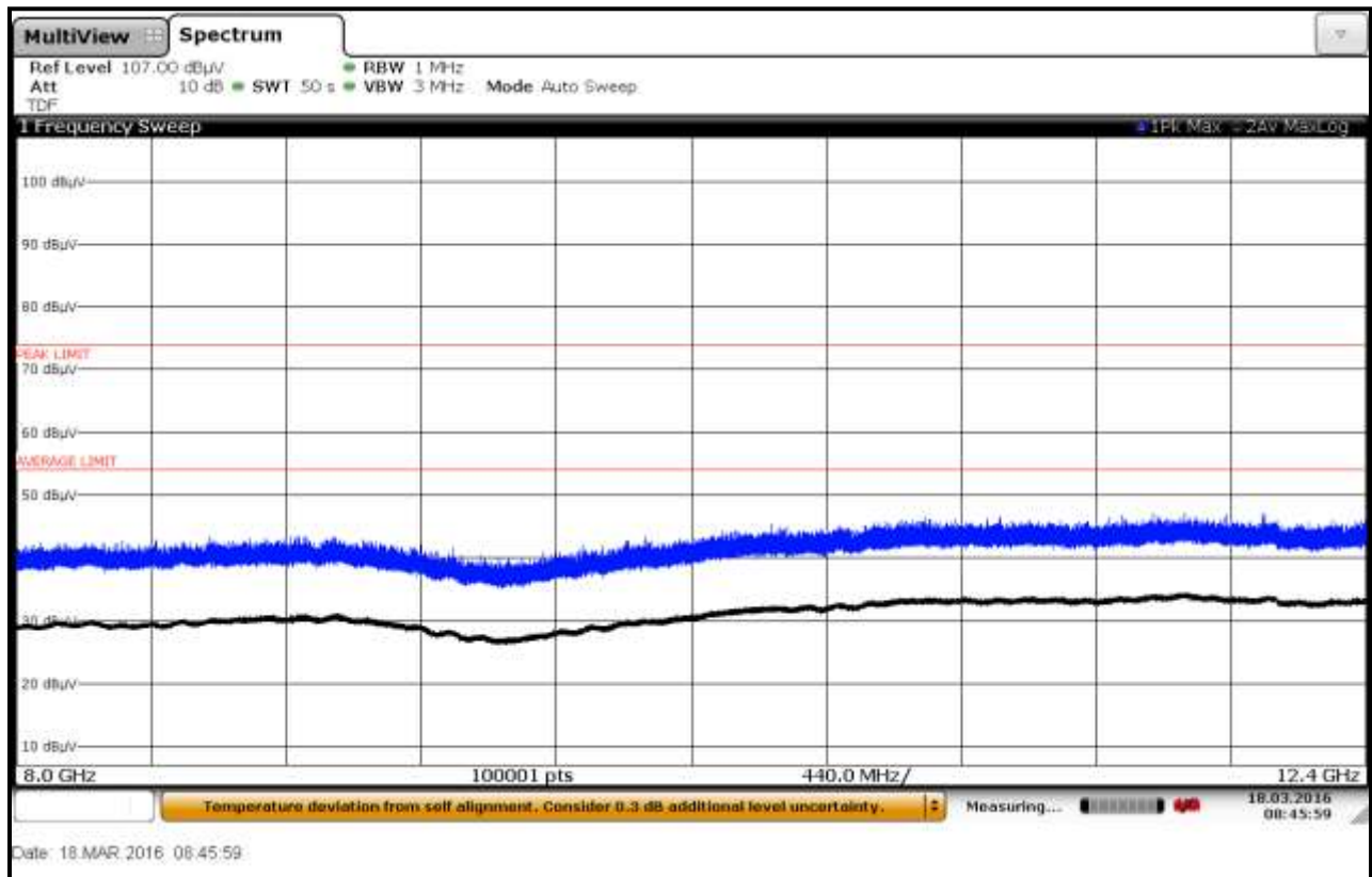
Plot 6-28: Radiated Emissions 8 GHz – 12.4 GHz; Fiberglass Container; TC #1, Horizontal
