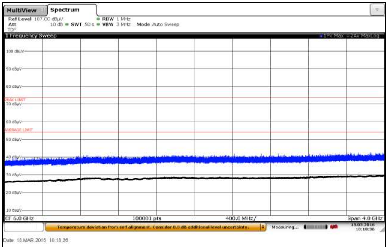
Plot 6-57: Radiated Emissions 4 GHz – 8 GHz; Fiberglass Container; TC #2; Vertical
