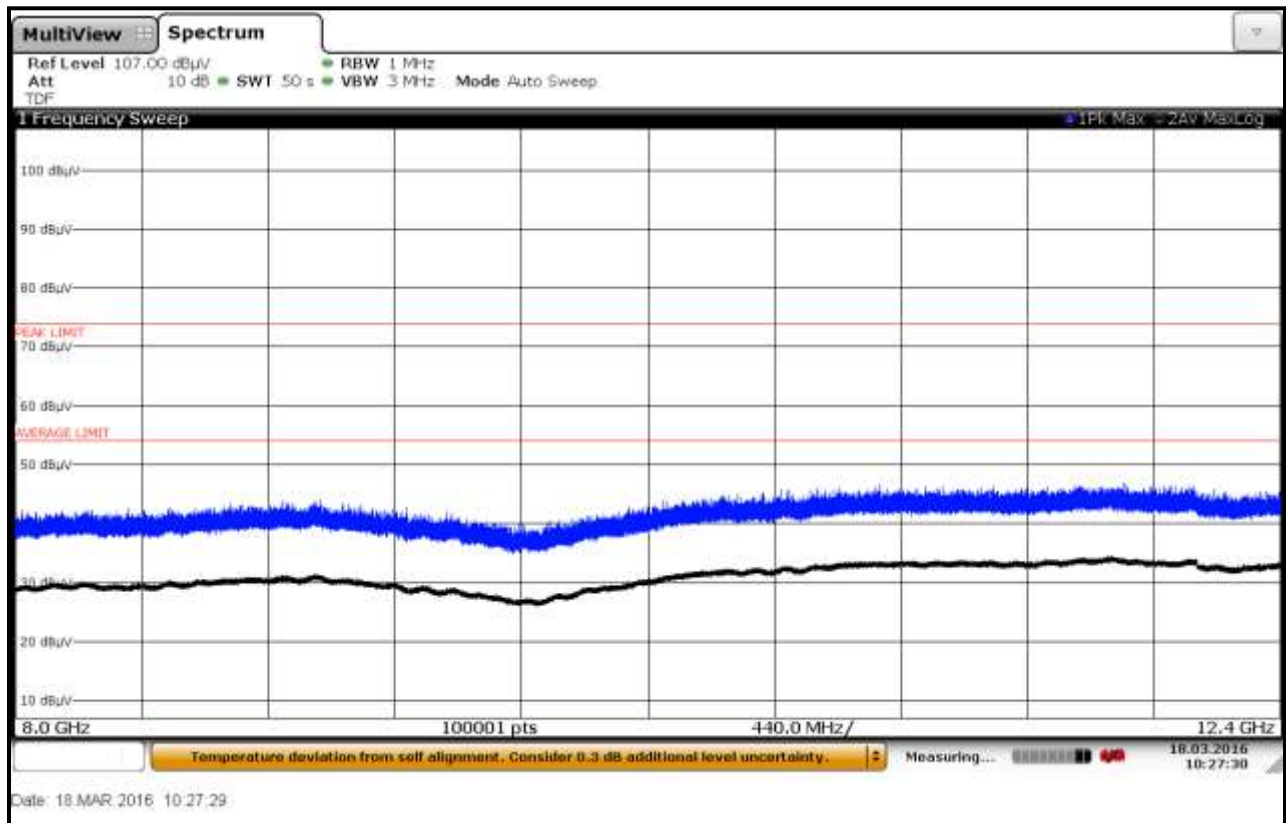
Plot 6-59: Radiated Emissions 8 GHz – 12.4 GHz; Fiberglass Container; TC #2, Vertical
