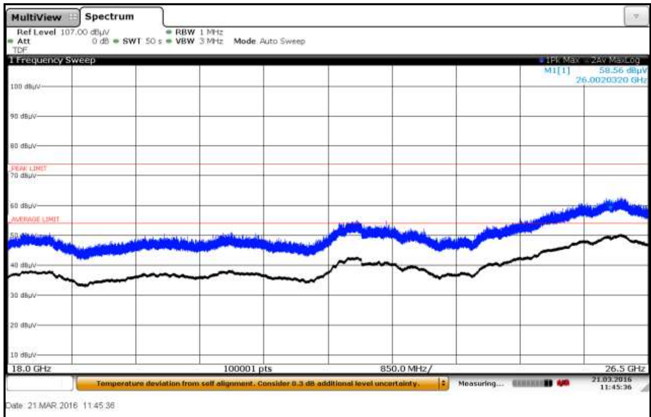
Plot 6-63: Radiated Emissions 18 GHz – 26.5 GHz; Fiberglass Container; TC #2, Vertical
