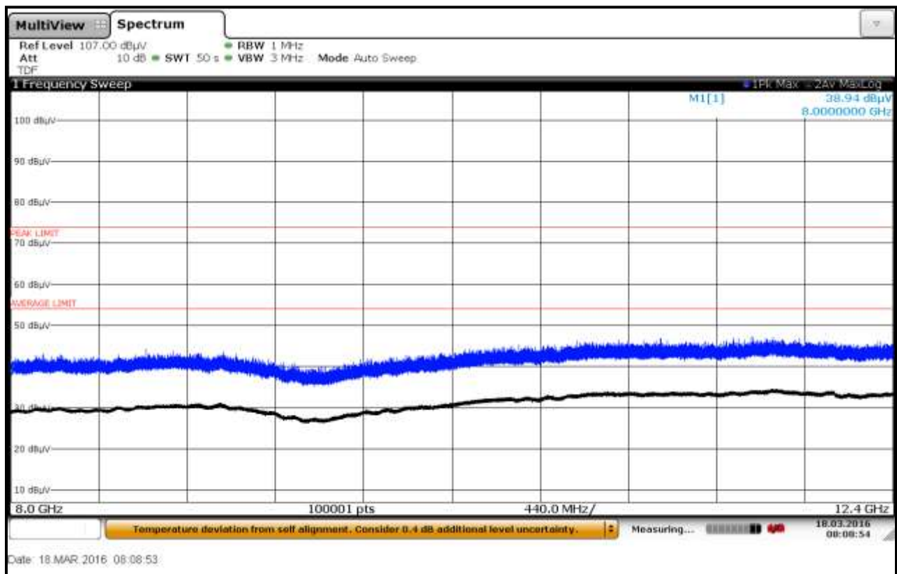
Plot 6-88: Radiated Emissions 8 GHz – 12.4 GHz; Fiberglass Container; TC #3, Horizontal
