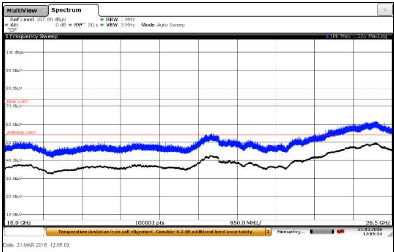
Plot 6-92: Radiated Emissions 18 GHz – 26.5 GHz; Fiberglass Container; TC #3, Horizontal
