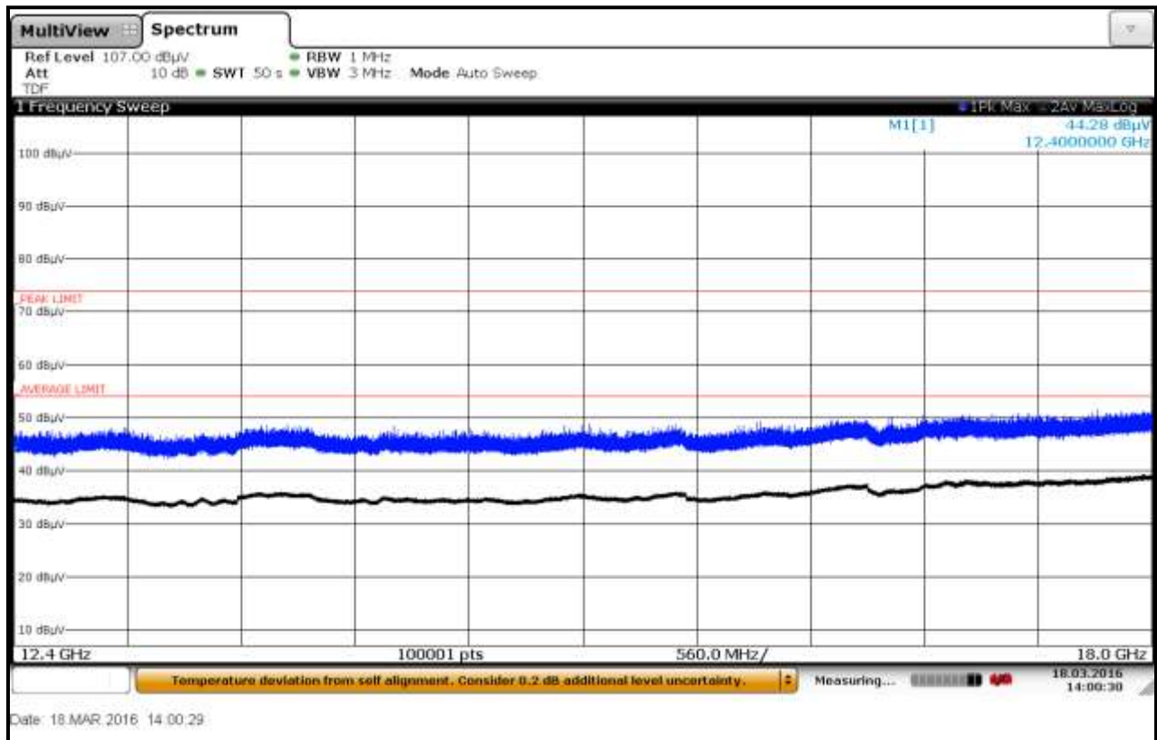
Plot 6-71: Radiated Emissions 12.4 GHz – 18 GHz; Metal Container; TC #3, Vertical
