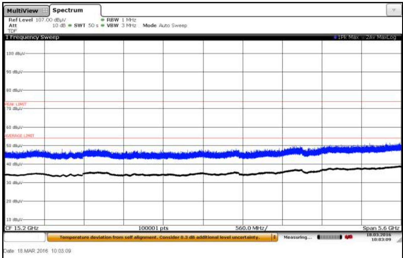
Plot 6-61: Radiated Emissions 12.4 GHz – 18 GHz; Fiberglass Container; TC #2, Vertical
