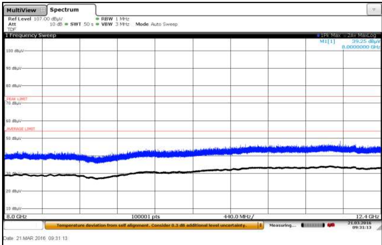
Plot 6-78: Radiated Emissions 8 GHz – 12.4 GHz; Concrete Container; TC #3, Horizontal
