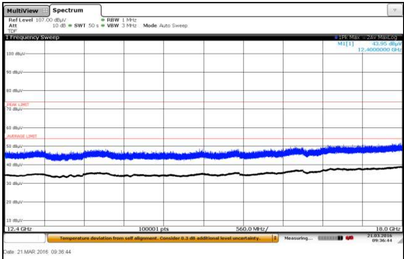
Plot 6-80: Radiated Emissions 12.4 GHz – 18 GHz; Concrete Container; TC #3, Horizontal
