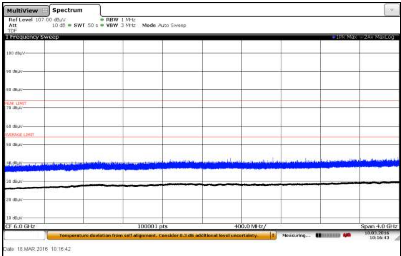
Plot 6-56: Radiated Emissions 4 GHz – 8 GHz; Fiberglass Container; TC #2; Horizontal
