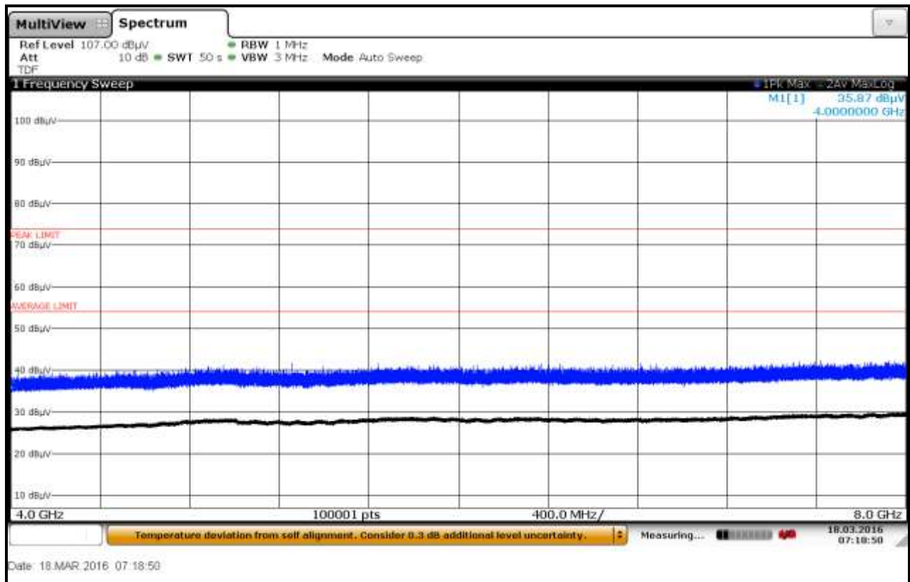
Plot 6-87: Radiated Emissions 4 GHz – 8 GHz; Fiberglass Container; TC #3; Vertical
