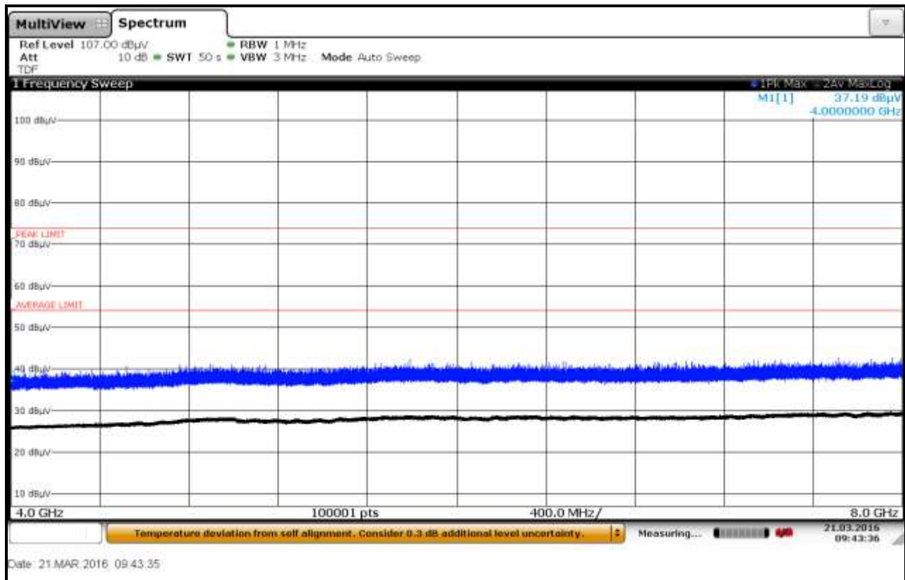
Plot 6-76: Radiated Emissions 4 GHz – 8 GHz; Concrete Container; TC #3; Horizontal
