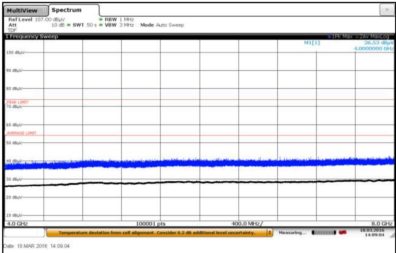
Plot 6-67: Radiated Emissions 4 GHz – 8 GHz; Metal Container; TC #3; Vertical
