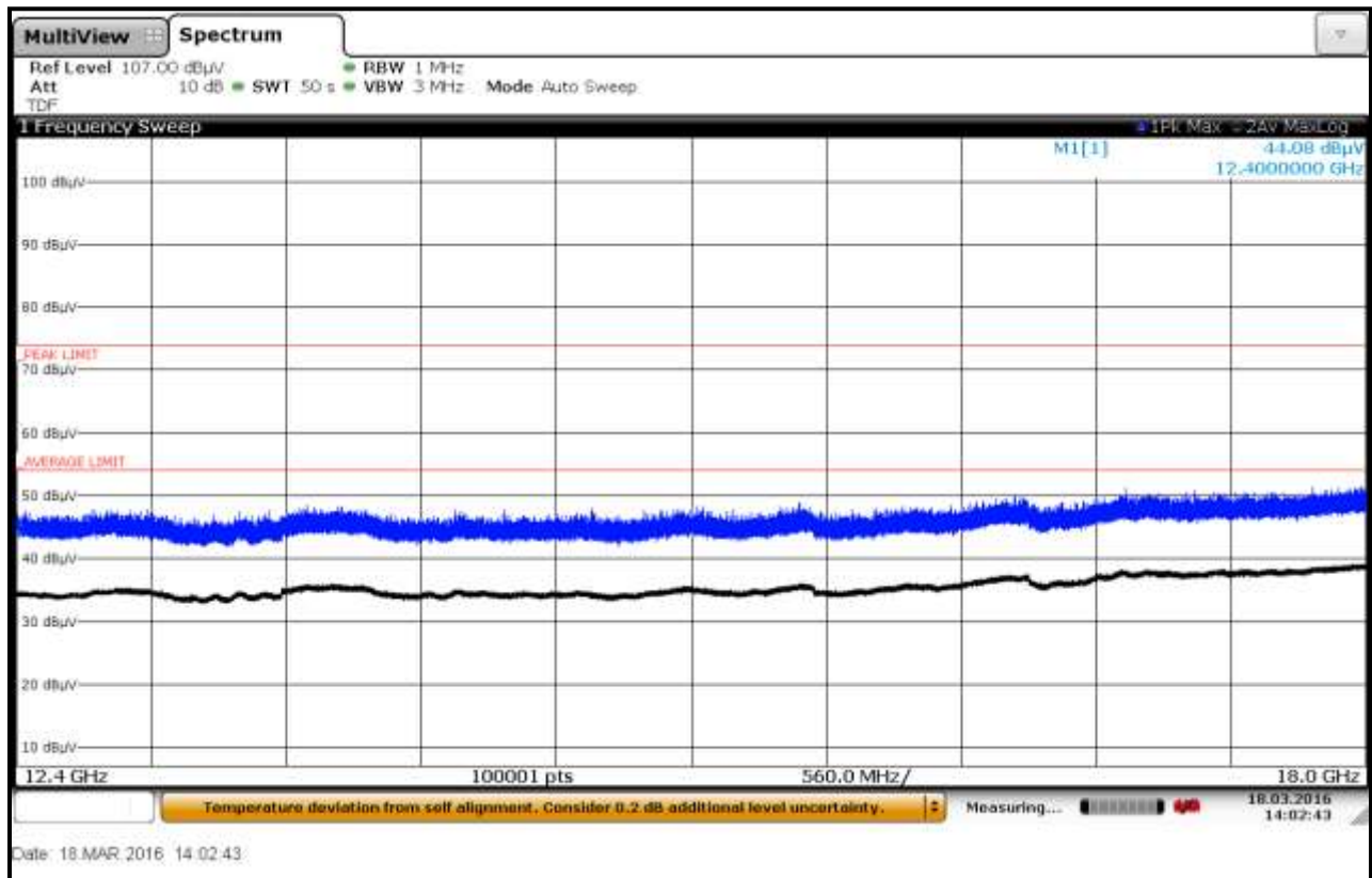
Plot 6-70: Radiated Emissions 12.4 GHz – 18 GHz; Metal Container; TC #3, Horizontal
