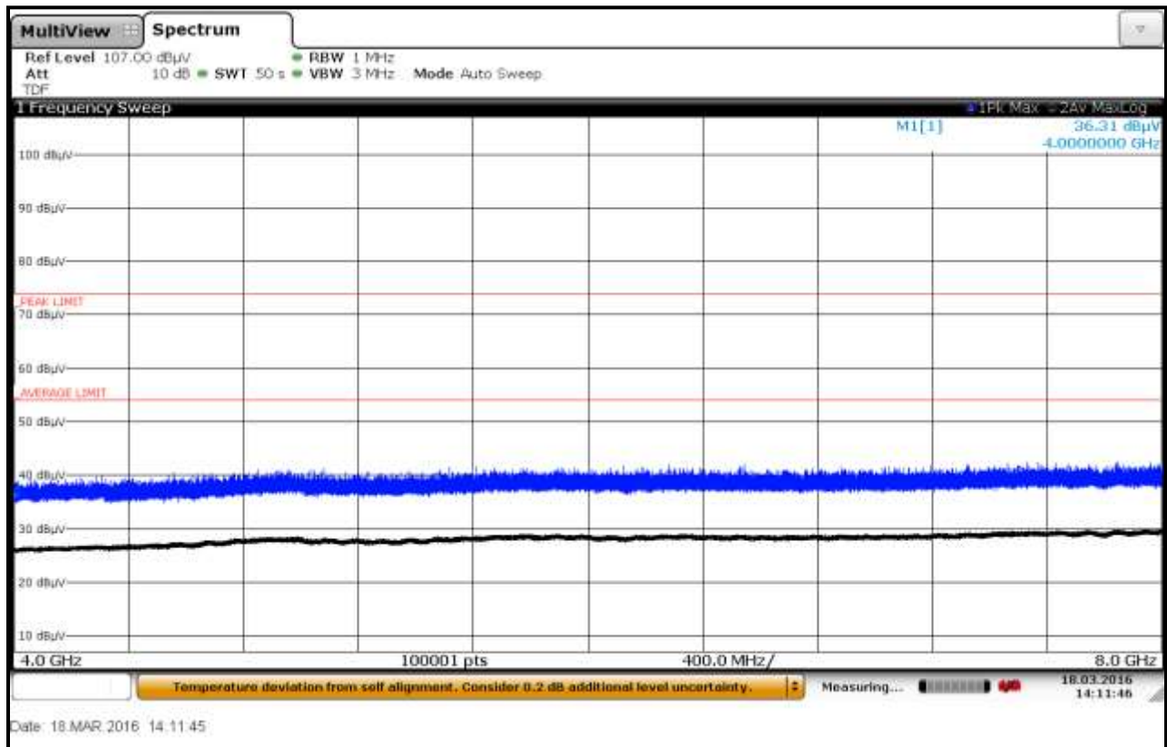
Plot 6-66: Radiated Emissions 4 GHz – 8 GHz; Metal Container; TC #3; Horizontal
