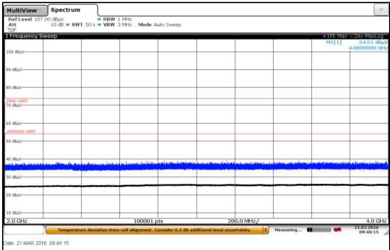
Plot 6-75: Radiated Emissions 2 GHz – 4 GHz; Concrete Container; TC #3; Vertical
