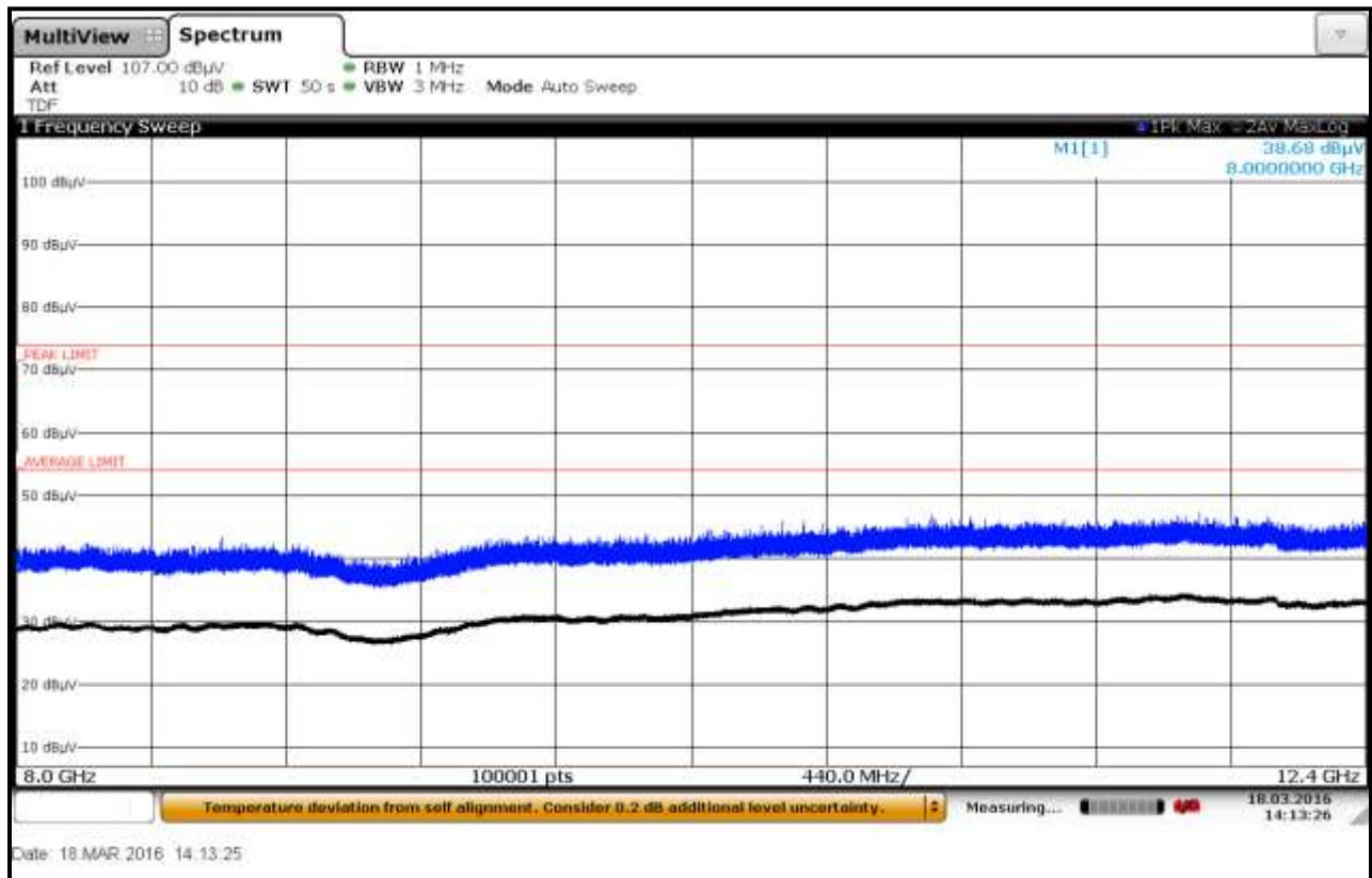
Plot 6-68: Radiated Emissions 8 GHz – 12.4 GHz; Metal Container; TC #3, Horizontal
