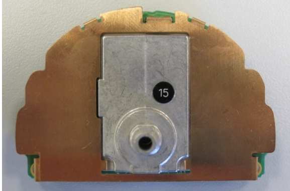
Top View with Shielding
