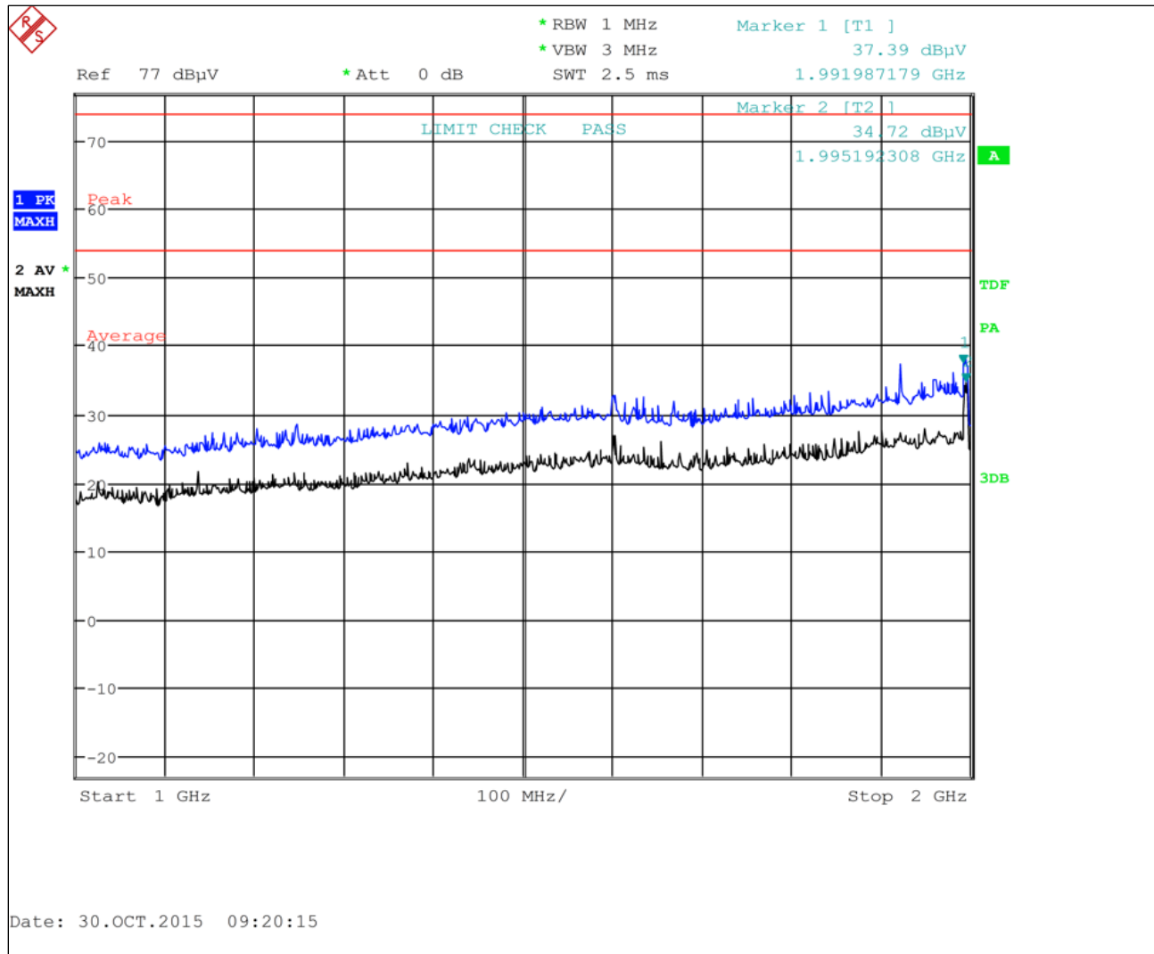
Plot 6-134: Radiated Emissions 1 GHz – 2 GHz Horizontal Peak/Average
