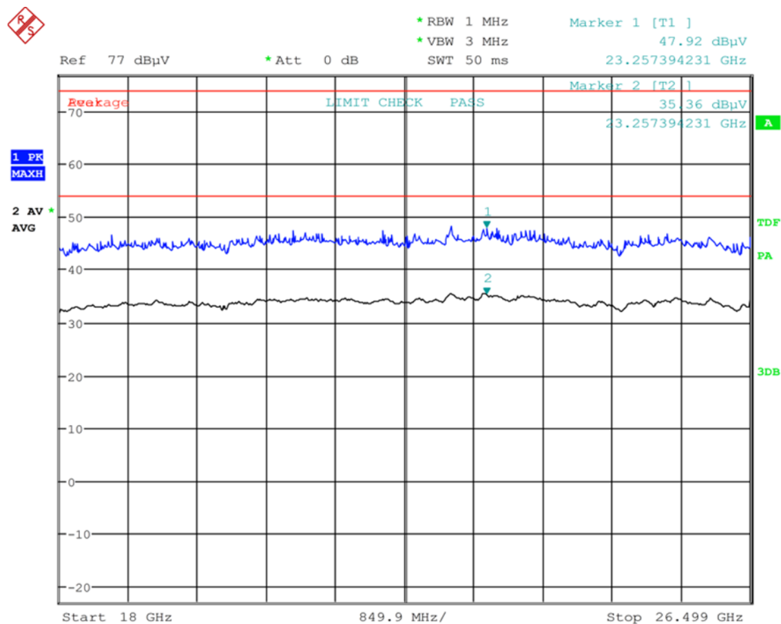
Plot 6-461: Radiated Emissions of Carrier - TC #5 Fiberglass Container
