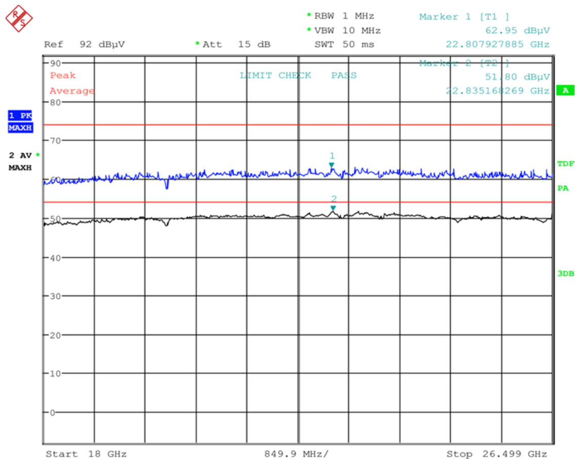
Plot 6-125: Radiated Emissions of Carrier - TC #7 Steel Container
