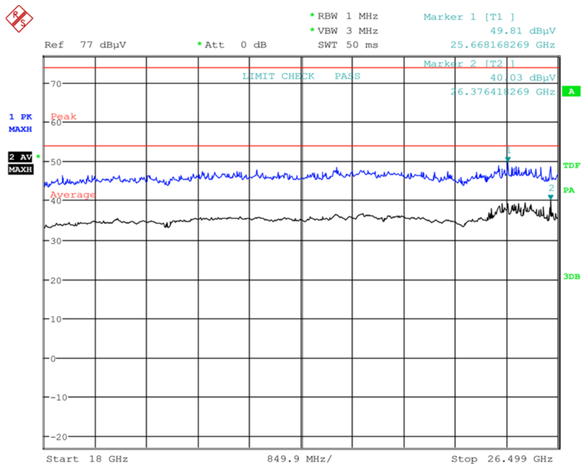
Plot 6-146: Radiated Emissions of Carrier - TC #8 Steel Container
