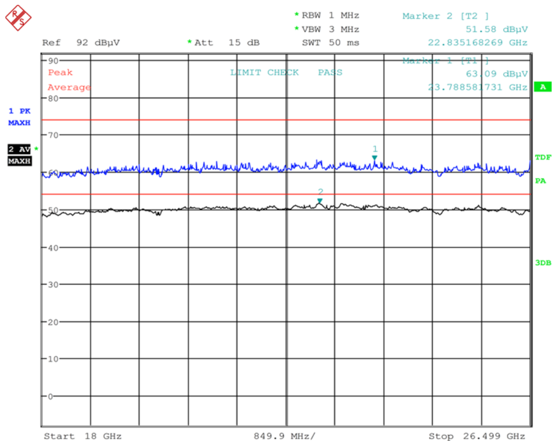
Plot 6-104: Radiated Emissions of Carrier - TC #6 Steel Container
