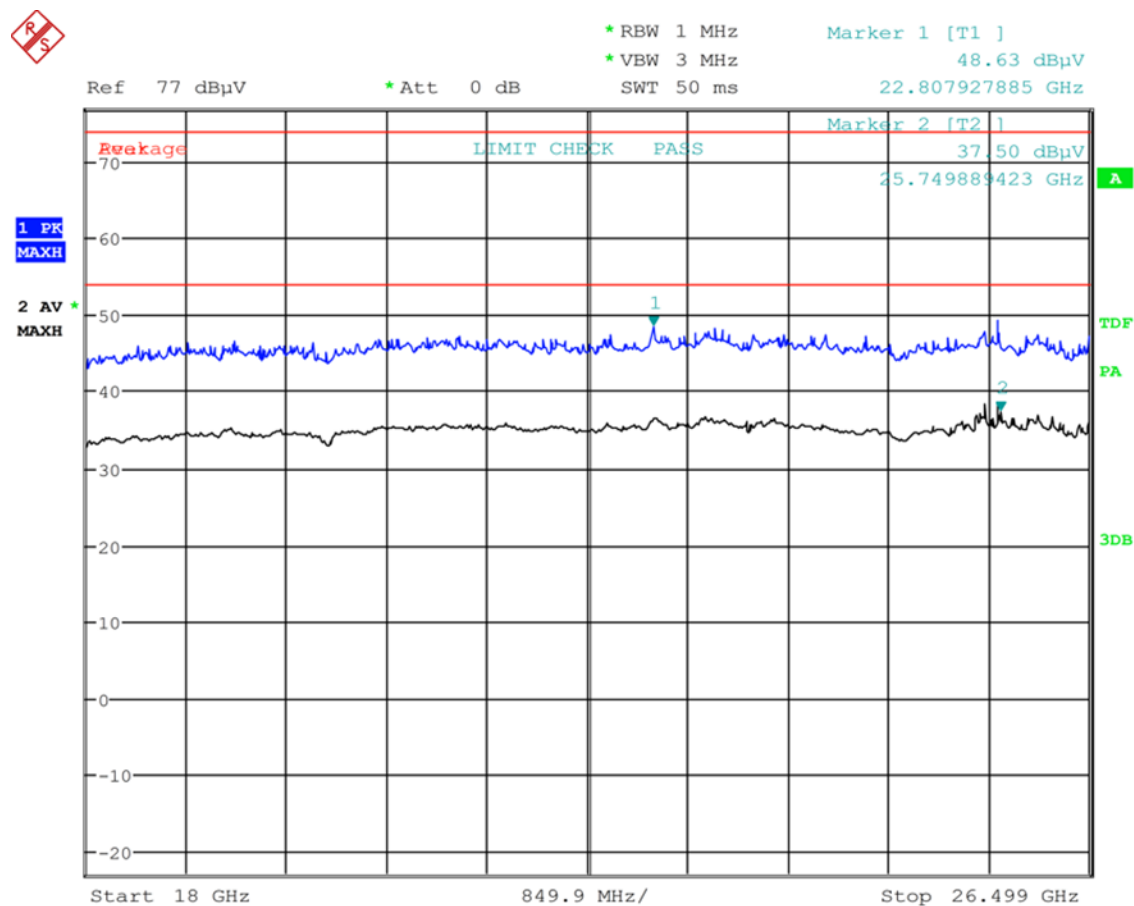
Plot 6-20: Radiated Emissions of Carrier - TC #2 Steel Container
