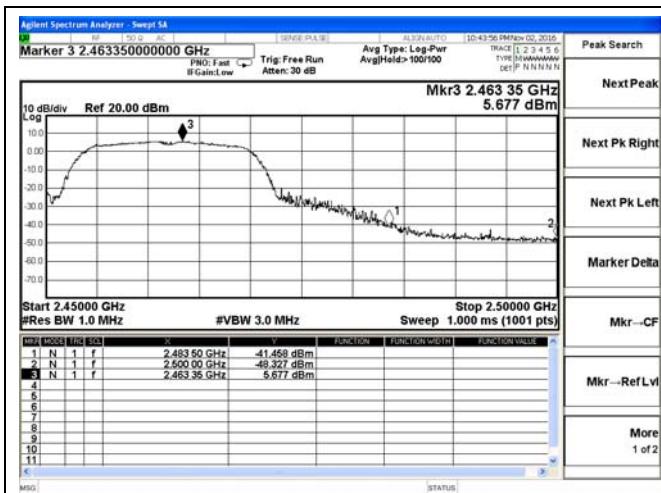
802.11g-High channel(Peak)
