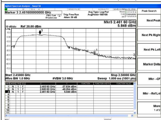
802.11n-HT20-High channel(Peak)
