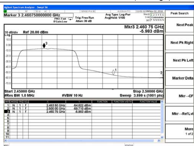
802.11n-HT20-High channel(Average)
