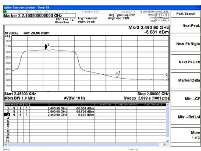
802.11g-High channel(Average)
