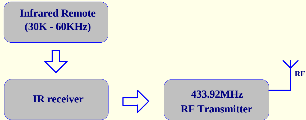
Block diagram of HIPRE01-TX (IR SENSOR / WIRELESS TRANSMITTER)
