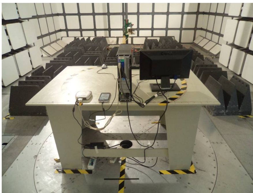
Radiated Emissions – Rear View (downloading mode, 1-5GHz)
