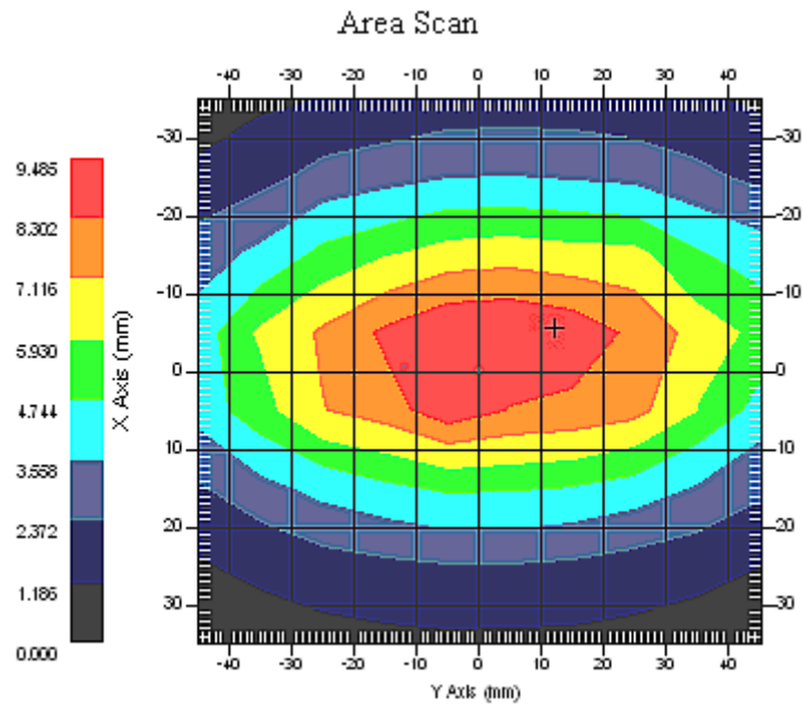
835 MHz System Validation with Body Tissue
